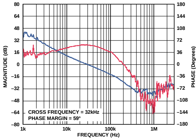
Figure 40. ADP2302 Bode Plot, V_{OUT} = 5\text{ V} , V_{IN} = 12\text{ V} , L = 6.8\text{ }\mu\text{H} , C_{OUT} = 2 \times 22\text{ }\mu\text{F}
