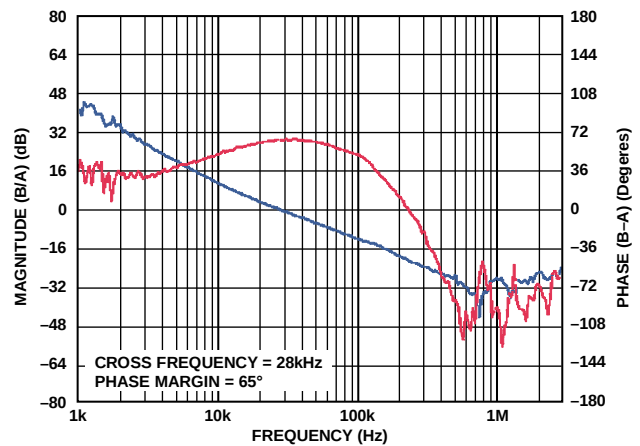
Figure 43. ADP2303 Bode Plot, V_{OUT} = 5\text{ V} , V_{IN} = 12\text{ V} , L = 4.7\text{ }\mu\text{H} , C_{OUT} = 47\text{ }\mu\text{F}
