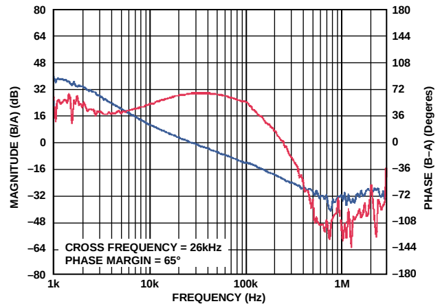
Figure 42. ADP2303 Bode Plot, V_{OUT} = 2.5\text{ V} , V_{IN} = 12\text{ V} , L = 3.3\text{ }\mu\text{H} , C_{OUT} = 2 \times 47\text{ }\mu\text{F}
