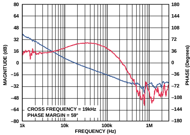
Figure 41. ADP2303 Bode Plot, V_{OUT} = 3.3\text{ V} , V_{IN} = 12\text{ V} , L = 4.7\text{ }\mu\text{H} , C_{OUT} = 2 \times 47\text{ }\mu\text{F}
