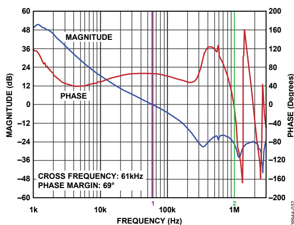
Figure 32. Bode Plot at V_{IN} = 5\text{ V} , V_{OUT} = 1.2\text{ V} , I_O = 4\text{ A} , f_s = 1.2\text{ MHz} , L = 0.68\text{ }\mu\text{H} , C_{OUT} = 47\text{ }\mu\text{F} + 100\text{ }\mu\text{F}
