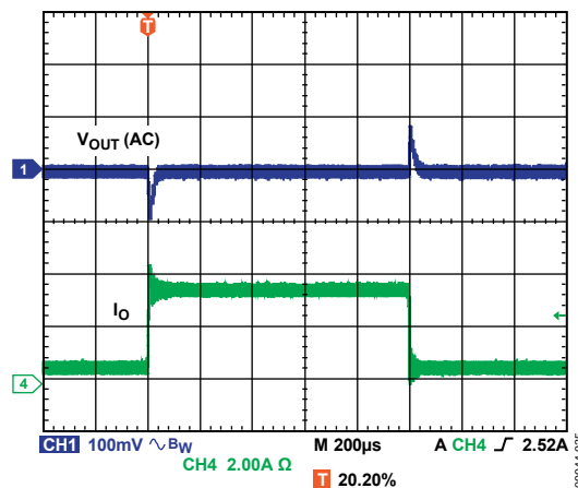
Figure 25. Load Transient, 0.5 A to 3.5 A Load Step, V_{IN} = 5\text{ V} , V_{OUT} = 1.2\text{ V} , f_s = 600\text{ kHz}
