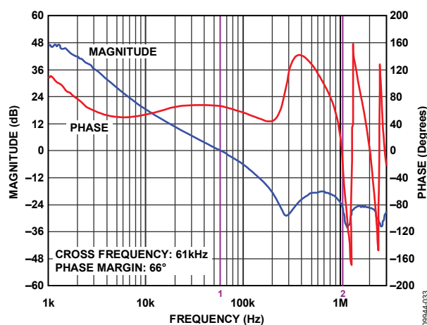
Figure 33. Bode Plot at V_{IN} = 5\text{ V} , V_{OUT} = 1.8\text{ V} , I_O = 4\text{ A} , f_s = 1.2\text{ MHz} , L = 1\text{ }\mu\text{H} , C_{OUT} = 100\text{ }\mu\text{F}
