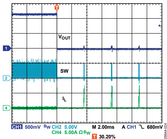
Figure 24. Output Short
