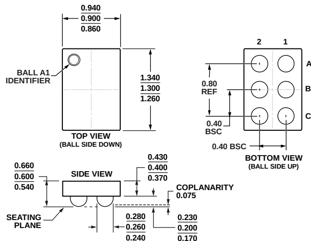
Figure 59. 6-Ball Wafer Level Chip Scale Package [WLCSP] (CB-6-4)
