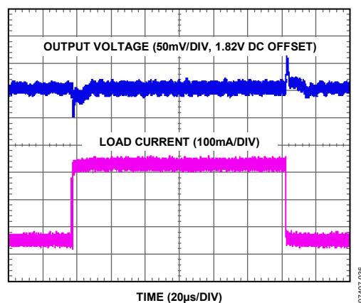
Figure 39. Load Transient Response, 150 mA to 400 mA ( V_{IN} = 4.5 V, PWM Mode)
