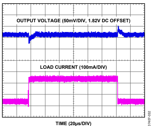
Figure 35. Load Transient Response, 50 mA to 250 mA ( V_{IN} = 3.6 V, PWM Mode)
