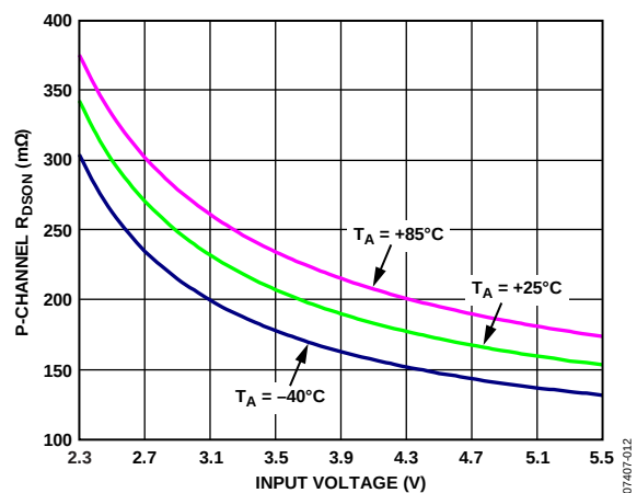
Figure 21. P-Channel Drain-Source On Resistance
