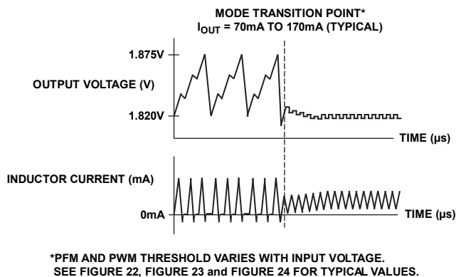
Figure 53. PFM-to-PWM Transition Point, V_{OUT} = 1.82\text{ V}
