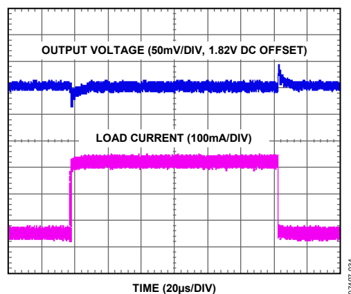
Figure 37. Load Transient Response, 150 mA to 400 mA ( V_{IN} = 2.5 V, PWM Mode)
