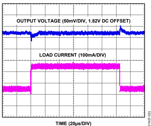
Figure 34. Load Transient Response, 50 mA to 250 mA ( V_{IN} = 2.5 V, PWM Mode)
