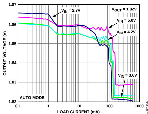
Figure 17. Output Voltage Accuracy (Auto Mode)
