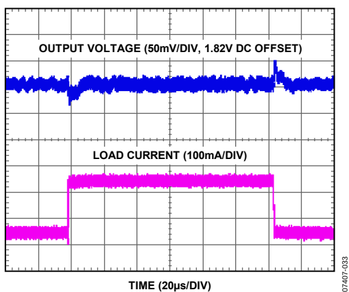
Figure 36. Load Transient Response, 50 mA to 250 mA ( V_{IN} = 4.5 V, PWM Mode)
