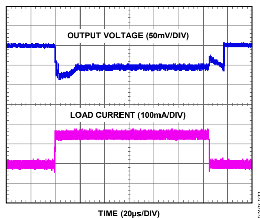
Figure 25. Load Transient Response, 0 mA to 150 mA ( V_{IN} = 2.5 V, Auto Mode)
