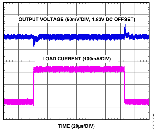
Figure 38. Load Transient Response, 150 mA to 400 mA ( V_{IN} = 3.6 V, PWM Mode)
