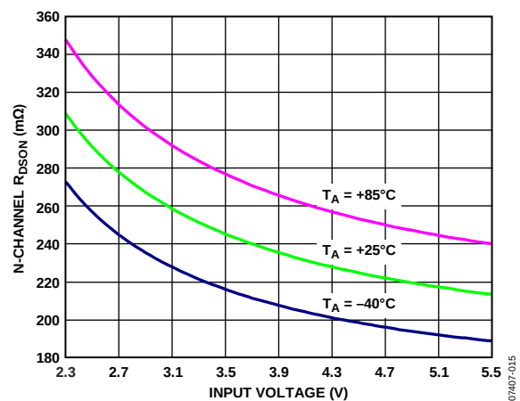
Figure 18. N-Channel Drain-Source On Resistance
