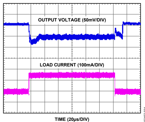
Figure 27. Load Transient Response, 0 mA to 150 mA ( V_{IN} = 4.5 V, Auto Mode)
