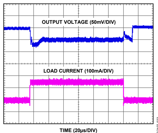
Figure 26. Load Transient Response, 0 mA to 150 mA ( V_{IN} = 3.6 V, Auto Mode)
