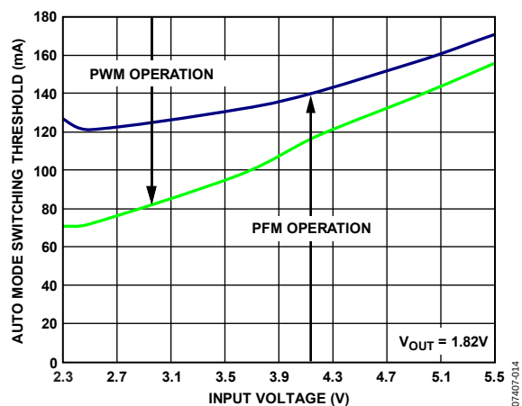
Figure 22. Auto Mode Switching Threshold vs. Input Voltage
