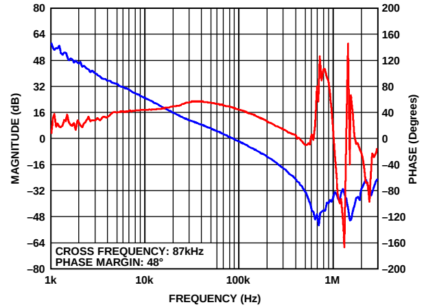
Figure 43. ADP2120 Bode Plot at V_{IN} = 5\text{ V} , V_{OUT} = 1.0\text{ V} , I_O = 1.25\text{ A} , L = 1.5\text{ }\mu\text{H} , C_{OUT} = 22\text{ }\mu\text{F} + 10\text{ }\mu\text{F}
