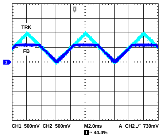
Figure 30. Tracking Function
