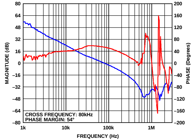
Figure 44. ADP2120 Bode Plot at V_{IN} = 5\text{ V} , V_{OUT} = 1.2\text{ V} , I_O = 1.25\text{ A} , L = 1.5\text{ }\mu\text{H} , C_{OUT} = 22\text{ }\mu\text{F} + 10\text{ }\mu\text{F}
