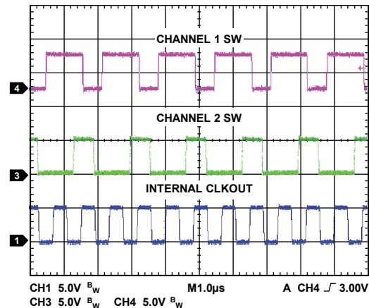
Figure 67. CLKOUT Waveforms
