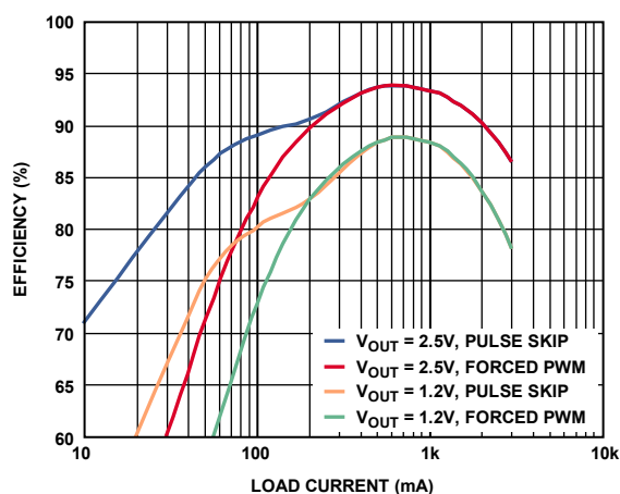
Figure 5. Efficiency vs. Load, V_{IN} = 5V and f_{SW} = 600 kHz ; V_{OUT} = 2.5V , Inductor TOKO FDV0620-3R3M, 3.3 \mu H , 40 m\Omega ; V_{OUT} = 1.2V , Inductor TOKO FDV0620-2R2M, 2.2 \mu H , 30 m\Omega
