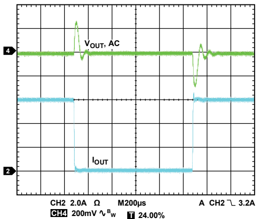
Figure 37. Load Transient Response in Forced PWM Mode, Combined Output: 0 A to 6 A Load Step, V_{IN} = 5 V, V_{OUT} = 3.3 V, f_{SW} = 600 kHz (See Table 12 for the Circuit Details)
