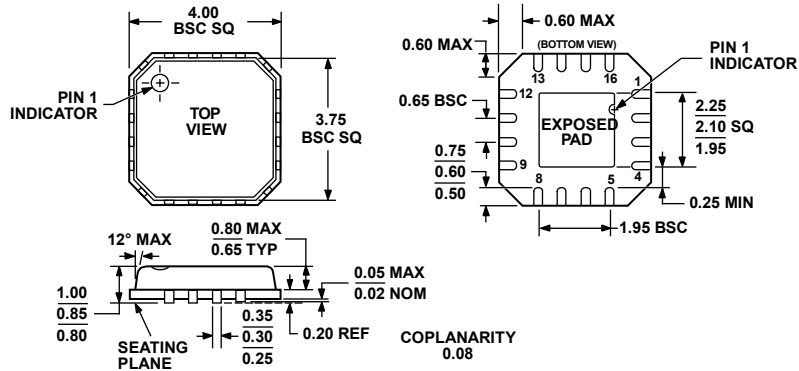
Figure 59. 16-Lead Lead Frame Chip Scale Package [LFCSP_VQ] 4 mm × 4 mm Body, Very Thin Quad (CP-16-4)
