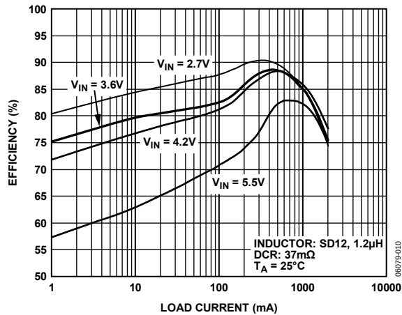
Figure 10. Efficiency—ADP2107 (1.2 V)
