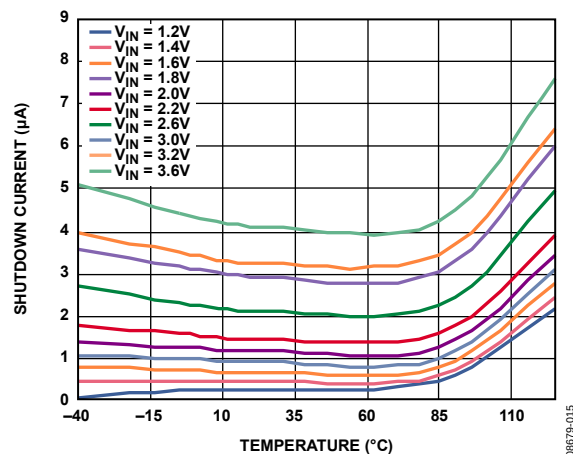
Figure 19. Reverse Output Shutdown Current vs. Temperature
