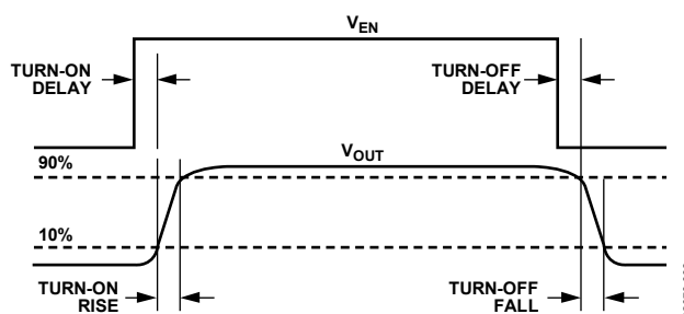
Figure 2. Timing Diagram
