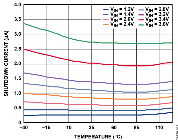
Figure 20. Reverse Shutdown Current vs. Temperature
