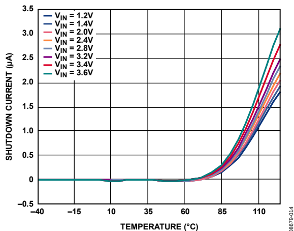
Figure 18. Reverse Input Shutdown Current vs. Temperature
