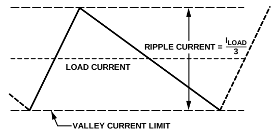
Figure 69. Valley Current Limit to Average Current Relation
