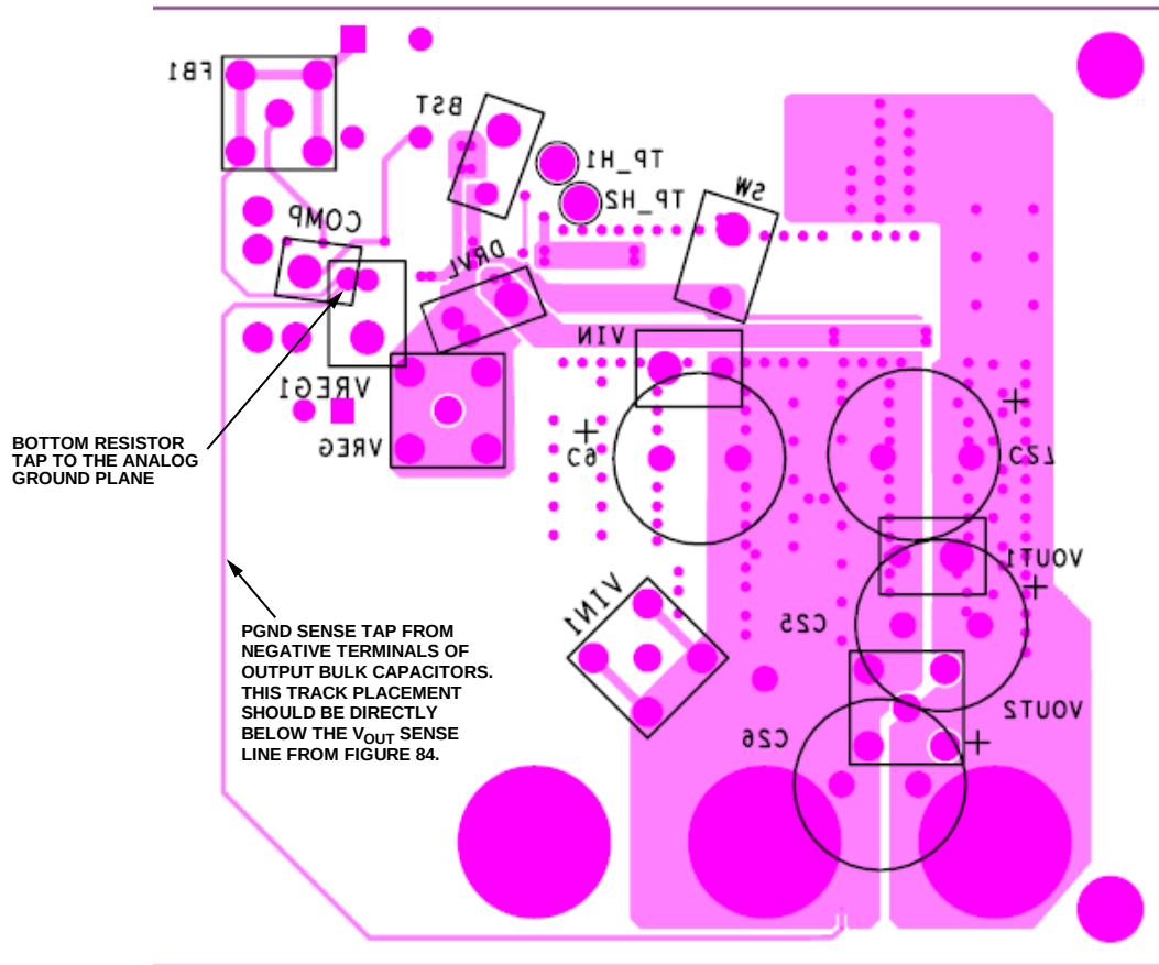
Figure 88. Layer 4 (Bottom Layer) of Evaluation Board
