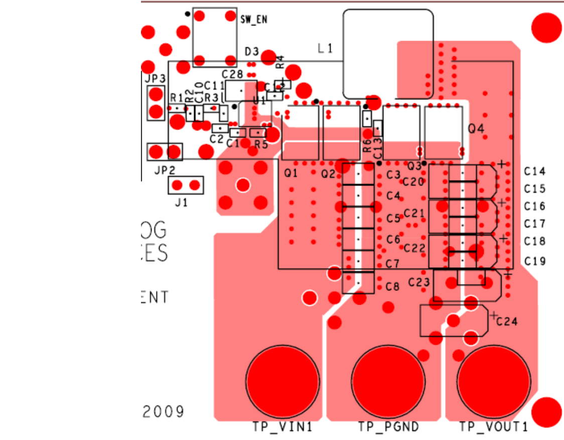
Figure 86. Layer 2 of Evaluation Board
