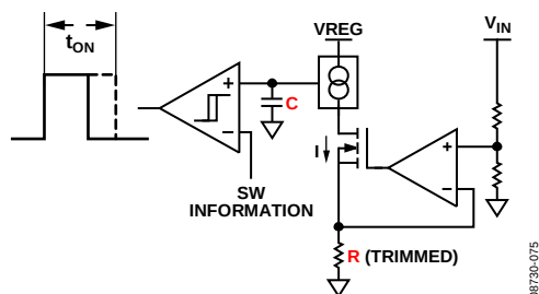
Figure 77. Constant On-Time
