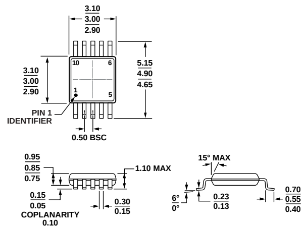
COMPLIANT TO JEDEC STANDARDS MO-187-BA Figure 94. 10-Lead Mini Small Outline Package [MSOP] (RM-10) Dimensions shown in millimeters
