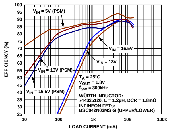
Figure 2. Efficiency vs. Load Current ( V_{OUT} = 1.8V , 300 kHz)
