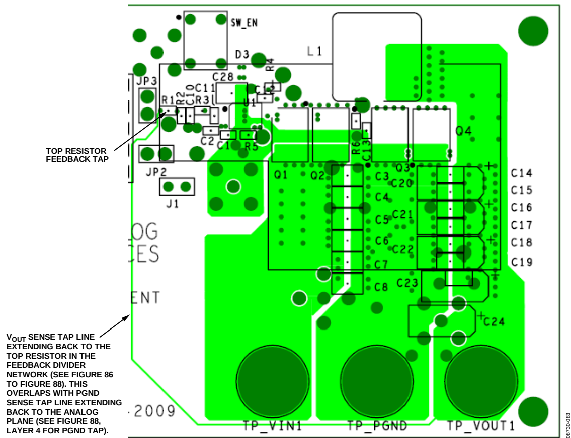
Figure 87. Layer 3 of Evaluation Board
