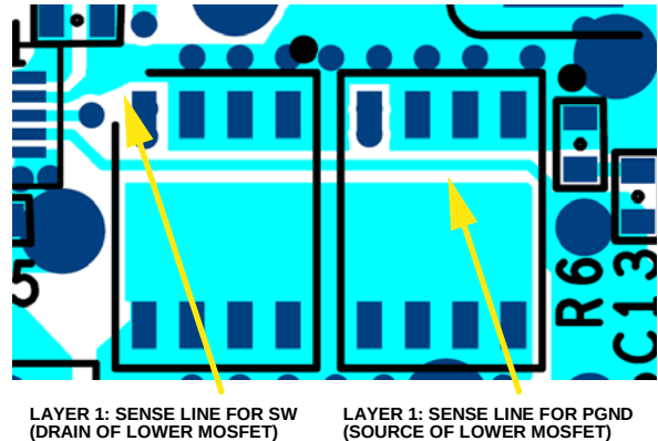
Figure 90. Drain/Source Tracking Tapping of the Lower-Side MOSFET for CS Amp Differential Sensing (Yellow Sense Line on Layer 2)
