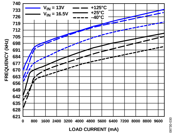
Figure 31. Frequency vs. Load Current, 600 kHz, V_{OUT} = 5\text{ V}
