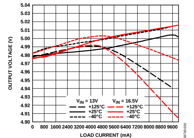
Figure 21. Output Voltage Accuracy—1.0 MHz, V_{OUT} = 5\text{ V}
