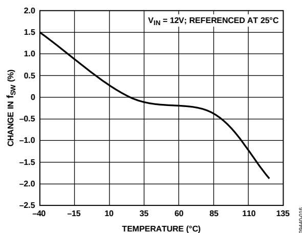
Figure 15. f_{SW} vs. Temperature
