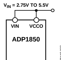
Figure 26. Configuration for V_{IN} < 5.5 V
