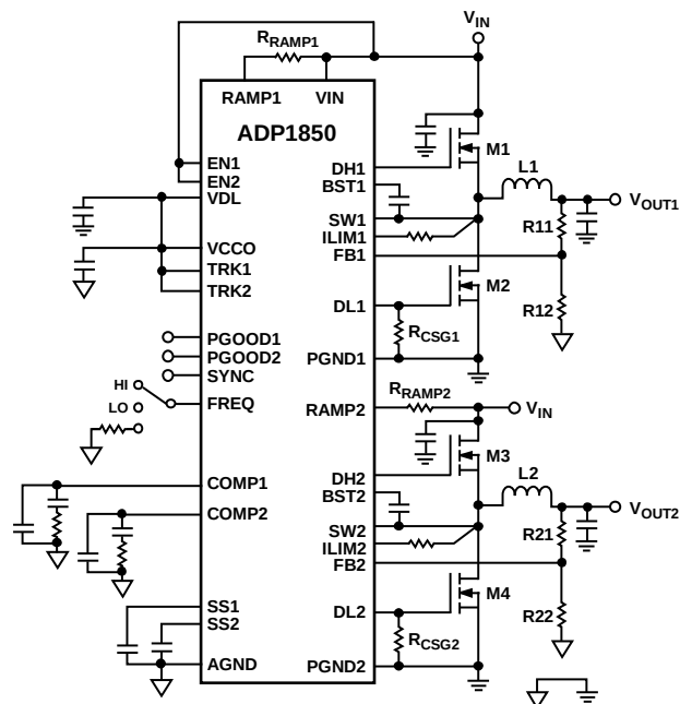
Figure 1. Single Phase Circuit
