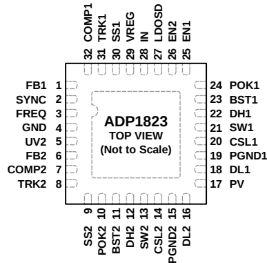
Figure 3. Pin Configuration
