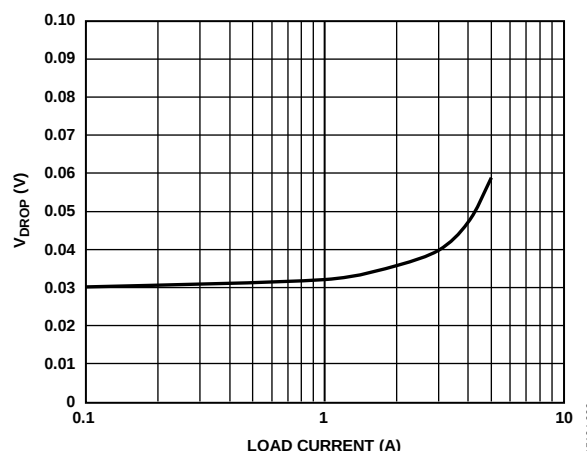
Figure 6. Dropout Voltage vs. Load Current, V_{OUT} = 1.3 V, T_A = 25^\circ\text{C}
