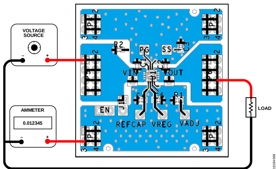
Figure 8. Ground Current Measurement Setup
