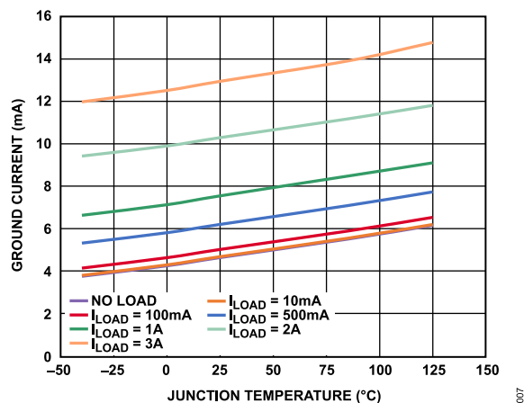
Figure 7. Ground Current ( I_{GND} ) vs. Junction Temperature ( T_J )
