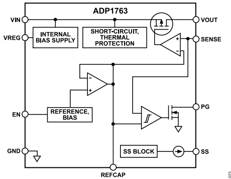
Figure 23. Functional Block Diagram, Fixed Output
