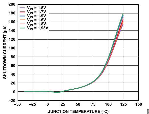
Figure 10. Shutdown Current ( I_{GND-SD} ) vs. Junction Temperature ( T_J ) at Various Input Voltages ( V_{IN} )
