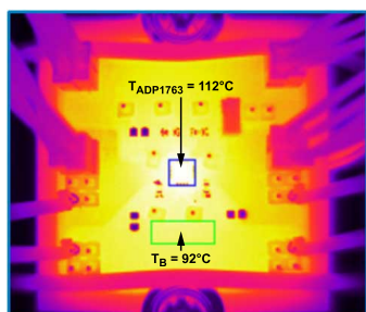
Figure 45. Thermal Image of the ADP1763 Evaluation Board at I_{LOAD} = 3\text{ A} , V_{IN} = 1.5\text{ V} , V_{OUT} = 1.3\text{ V} , T_B = 92^\circ\text{C}
