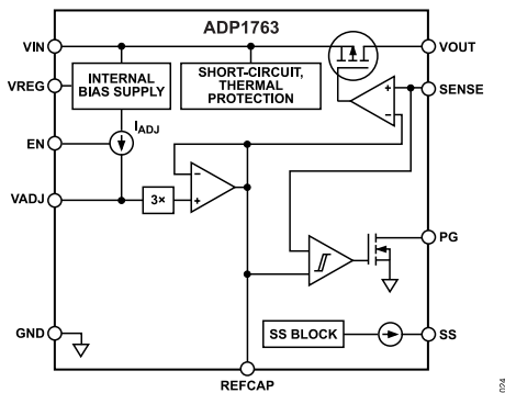
Figure 24. Functional Block Diagram, Adjustable Output
