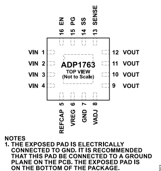
Figure 3. Pin Configuration
