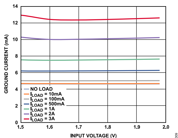
Figure 9. Ground Current ( I_{GND} ) vs. Input Voltage ( V_{IN} )
