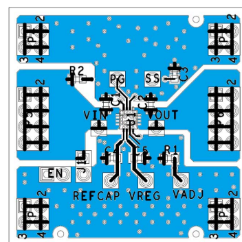
Figure 47. Typical Board Layout, Top Side
