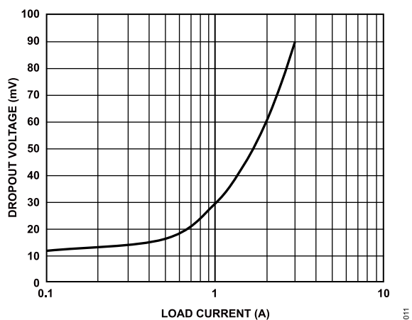
Figure 11. Dropout Voltage ( V_{DROP-OUT} ) vs. Load Current ( I_{LOAD} ), V_{OUT} = 1.3 V
