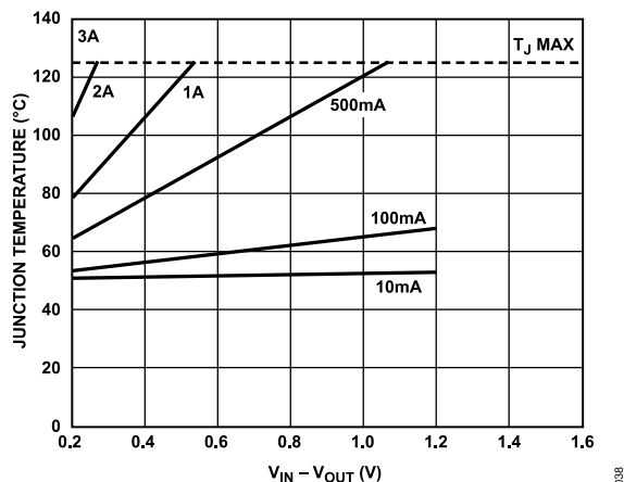
Figure 40. 25 mm² of PCB Copper, T_A = 50^\circ\text{C}
