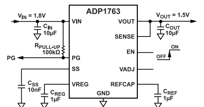
Figure 1. Fixed Output Operation
