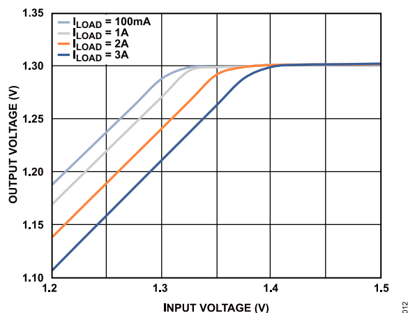
Figure 12. Output Voltage ( V_{OUT} ) vs. Input Voltage ( V_{IN} ) (in Dropout), V_{OUT} = 1.3 V
