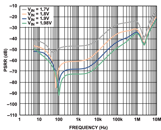
Figure 21. Power Supply Rejection Ratio (PSRR) vs. Frequency for Various Input Voltages, V_{OUT} = 1.5 V, Load Current = 3 A
