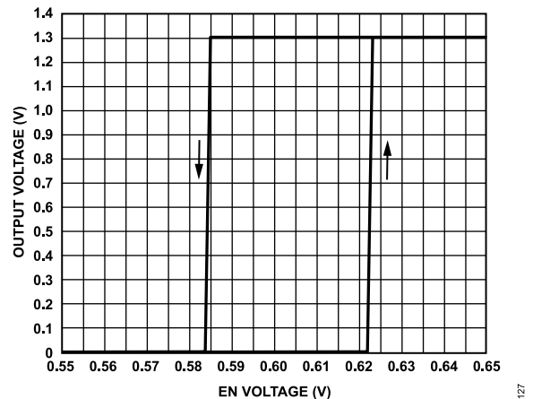
Figure 28. Output Voltage vs. Typical EN Pin Voltage, V_{OUT} = 1.3 V
