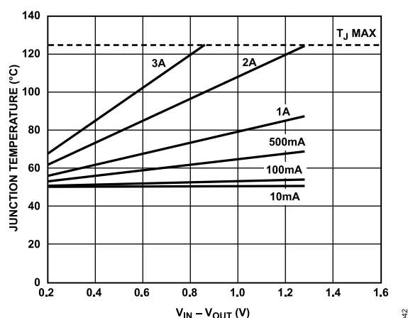
Figure 44. 1000 mm² of PCB Copper, T_B = 50^\circ\text{C} , LFCSP
