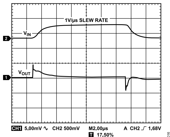
Figure 16. Line Transient Response, Load Current = 3 A, V_{IN} = 1.5 V to 1.98 V Step, V_{OUT} = 1.3 V
