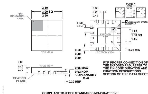
Figure 49. 16-Lead Lead Frame Chip Scale Package [LFCSP] 3 mm x 3 mm Body and 0.75 mm Package Height (CP-16-22) Dimensions shown in millimeters
