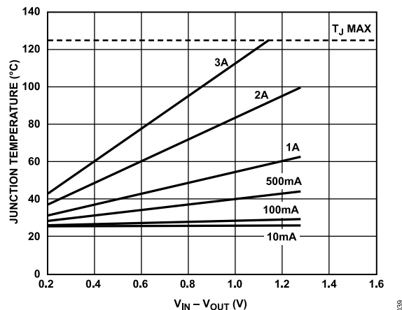
Figure 41. 500 mm² of PCB Copper, T_B = 25^\circ\text{C}
