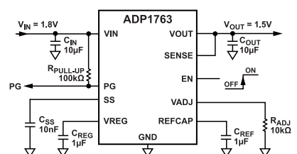
Figure 2. Adjustable Output Operation
