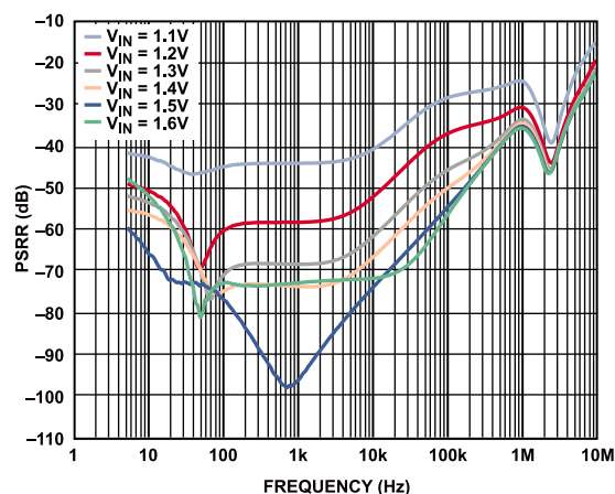
Figure 19. Power Supply Rejection Ratio (PSRR) vs. Frequency for Various Input Voltages, V_{OUT} = 0.9 V, Load Current = 3 A
