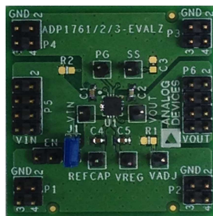
Figure 46. Evaluation Board
