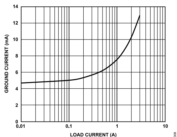
Figure 8. Ground Current ( I_{GND} ) vs. Load Current ( I_{LOAD} )
