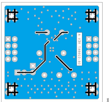
Figure 48. Typical Board Layout, Bottom Side
