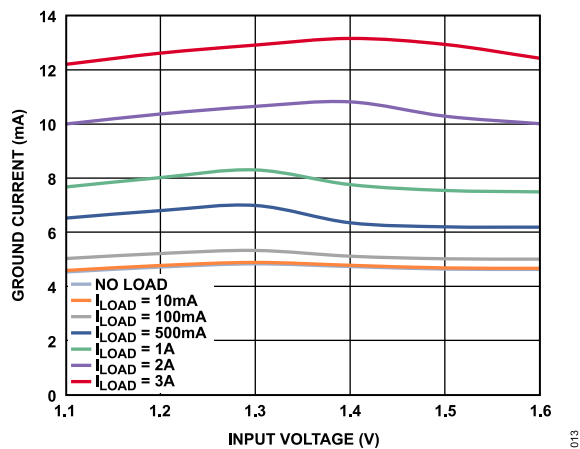
Figure 13. Ground Current ( I_{GND} ) vs. Input Voltage ( V_{IN} ) (in Dropout), V_{OUT} = 1.3 V
