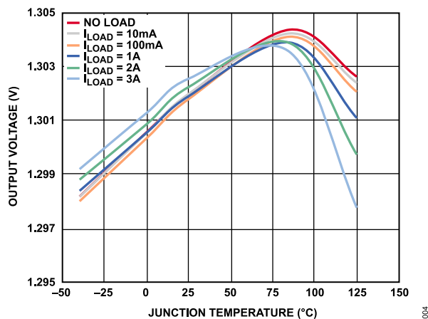
Figure 4. Output Voltage ( V_{OUT} ) vs. Junction Temperature ( T_J )
