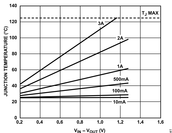
Figure 43. 1000 mm² of PCB Copper, T_B = 25^\circ\text{C}
