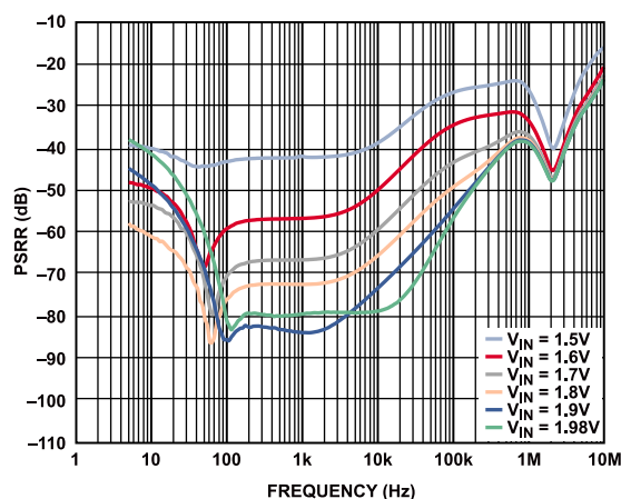
Figure 20. Power Supply Rejection Ratio (PSRR) vs. Frequency for Various Input Voltages, V_{OUT} = 1.3 V, Load Current = 3 A
