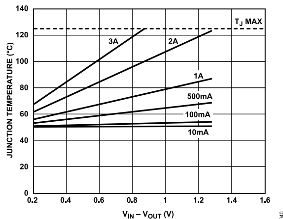
Figure 42. 500 mm² of PCB Copper, T_B = 50^\circ\text{C}
