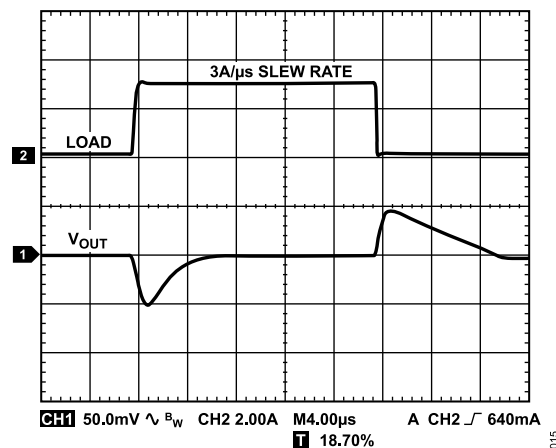
Figure 15. Load Transient Response, C_{OUT} = 47 \mu F , V_{IN} = 1.8 V , V_{OUT} = 1.3 V
