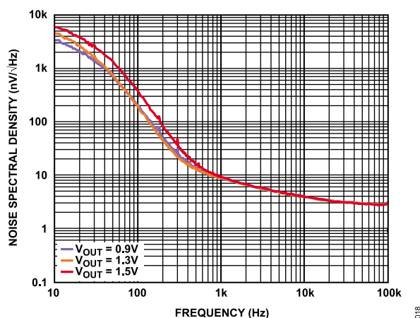
Figure 18. Noise Spectral Density vs. Frequency for Various Output Voltages, I_{LOAD} = 100 mA
