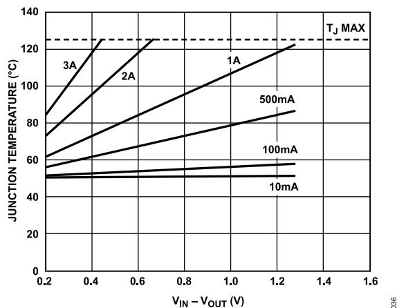
Figure 38. 6400 mm² of PCB Copper, T_A = 50^\circ\text{C}
