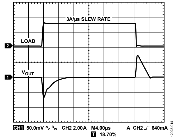
Figure 14. Load Transient Response, C_{OUT} = 10 \mu F , V_{IN} = 1.8 V , V_{OUT} = 1.3 V
