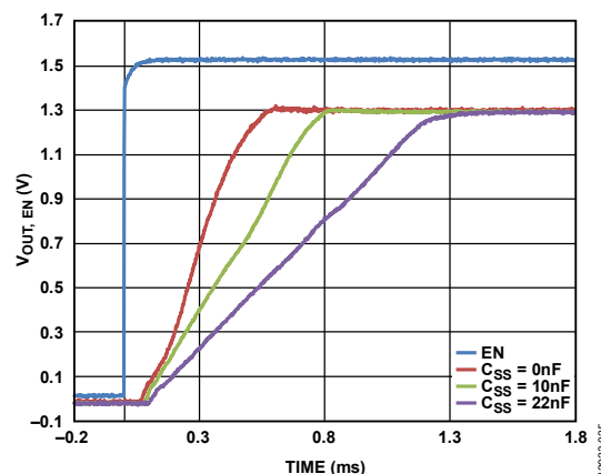
Figure 25. Fixed V_{OUT} Ramp-Up with External Soft Start Capacitor ( V_{OUT,EN} ) vs. Time
