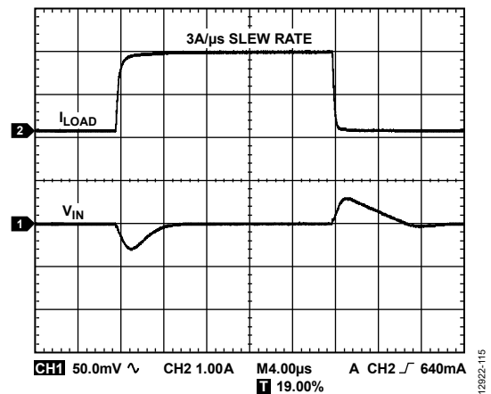
Figure 15. Load Transient Response, C_{OUT} = 47\text{ }\mu\text{F} , V_{IN} = 1.7\text{ V} , V_{OUT} = 1.3\text{ V}
