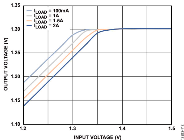
Figure 12. Output Voltage vs. Input Voltage (in Dropout), V_{OUT} = 1.3\text{ V}
