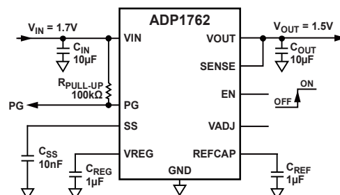
Figure 1. Fixed Output Operation
