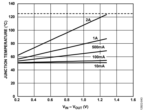
Figure 43. 1000 mm² of PCB Copper, T_B = 50^\circ\text{C}
