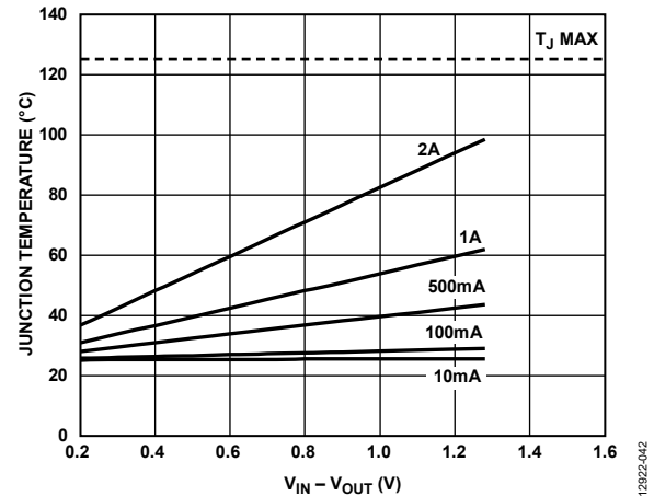
Figure 42. 1000 mm² of PCB Copper, T_B = 25^\circ\text{C}
