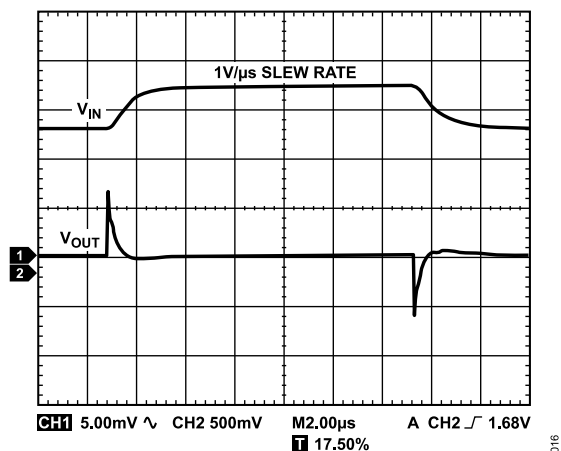
Figure 16. Line Transient Response, Load Current = 1 A, V_{IN} = 1.5 V to 1.98 V Step, V_{OUT} = 1.3 V
