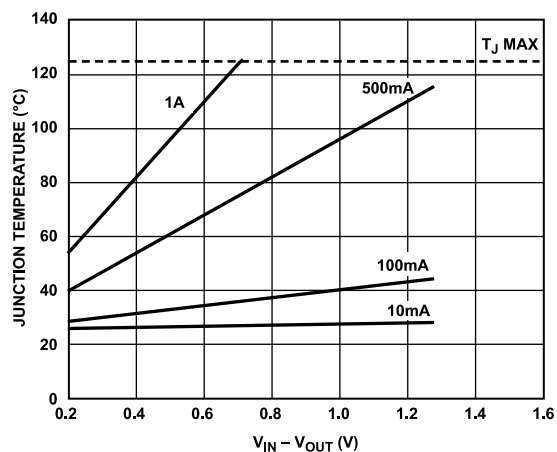
Figure 36. 25 mm² of PCB Copper, T_A = 25^\circ\text{C}
