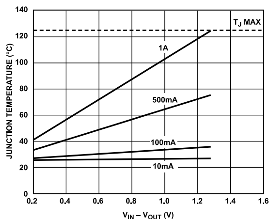
Figure 35. 500 mm² of PCB Copper, T_A = 25^\circ\text{C}
