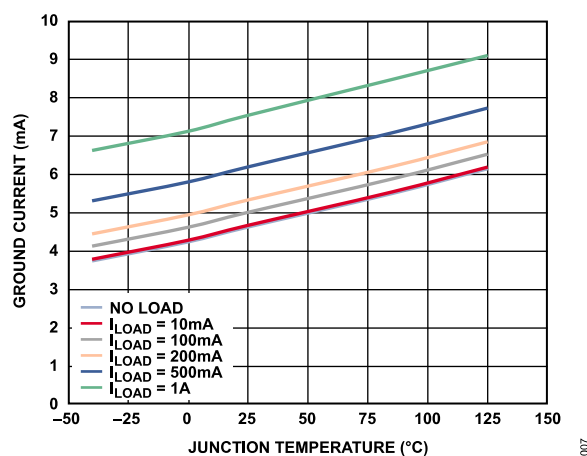
Figure 7. Ground Current ( I_{GND} ) vs. Junction Temperature ( T_J )
