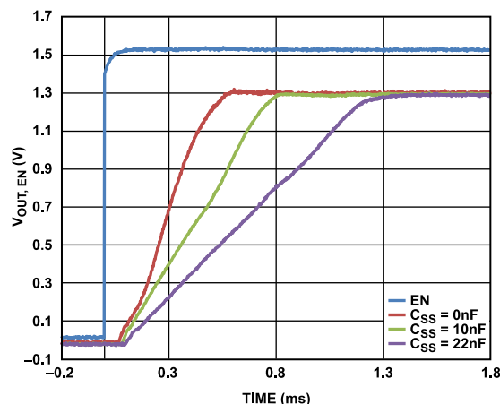
Figure 25. Fixed V_{\text{OUT}} Ramp-Up with External Soft Start Capacitor ( V_{\text{OUT}} , \text{EN} ) vs. Time
