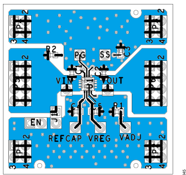
Figure 45. Typical Board Layout, Top Side
