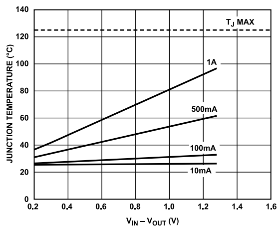
Figure 34. 6400 mm² of PCB Copper, T_A = 25^\circ\text{C}
