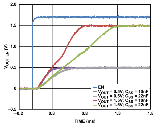
Figure 26. Adjustable V_{\text{OUT}} Ramp-Up with External Soft Start Capacitor ( V_{\text{OUT}} , \text{EN} ) vs. Time
