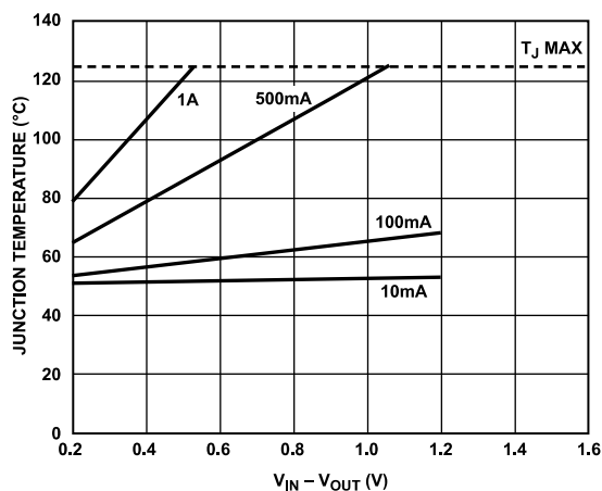
Figure 39. 25 mm² of PCB Copper, T_A = 50^\circ\text{C}
