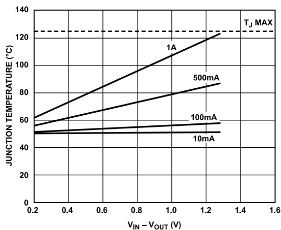
Figure 37. 6400 mm² of PCB Copper, T_A = 50^\circ\text{C}
