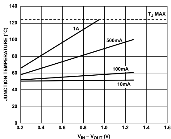
Figure 38. 500 mm² of PCB Copper, T_A = 50^\circ\text{C}
