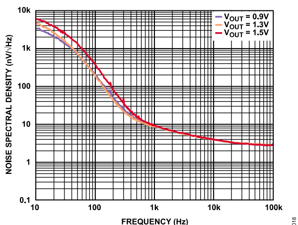
Figure 18. Noise Spectral Density vs. Frequency for Various Output Voltages, Load Current = 100 mA
