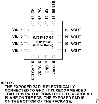
Figure 3. Pin Configuration
