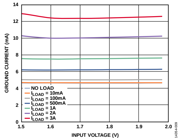
Figure 7. Ground Current vs. Input Voltage, V_{OUT} = 1.3 V, T_A = 25^\circ\text{C}
