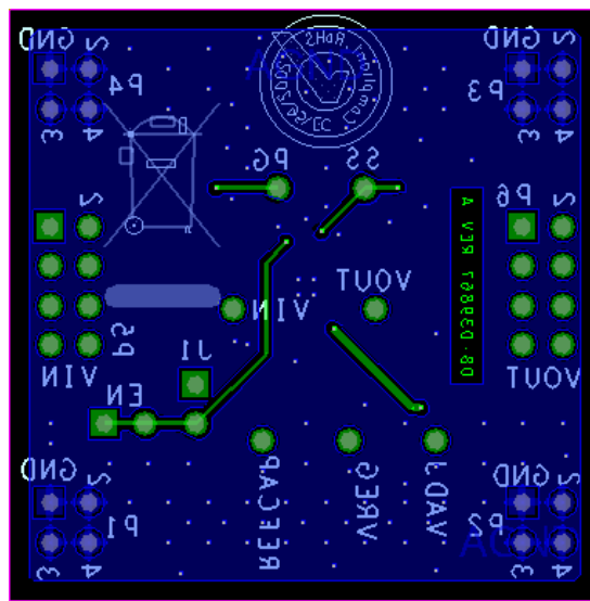
Figure 12. Bottom Layer
