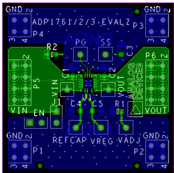
Figure 11. Top Layer
