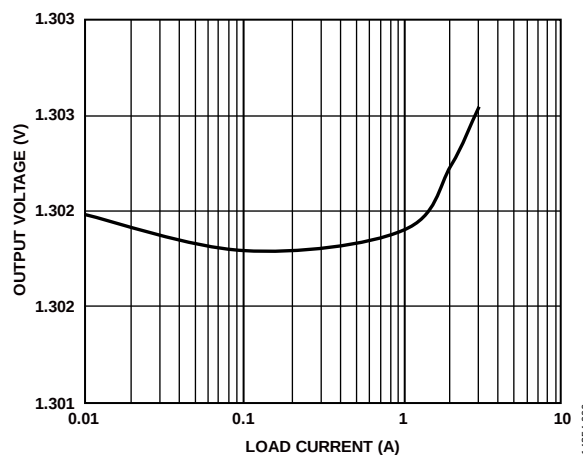
Figure 5. Output Voltage vs. Load Current at V_{IN} = 1.5 V, V_{OUT} = 1.3 V, T_A = 25^\circ\text{C}
