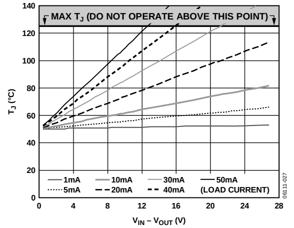
Figure 27. 0 \text{mm}^2 of PCB Copper, T_A = 50^{\circ}\text{C}
