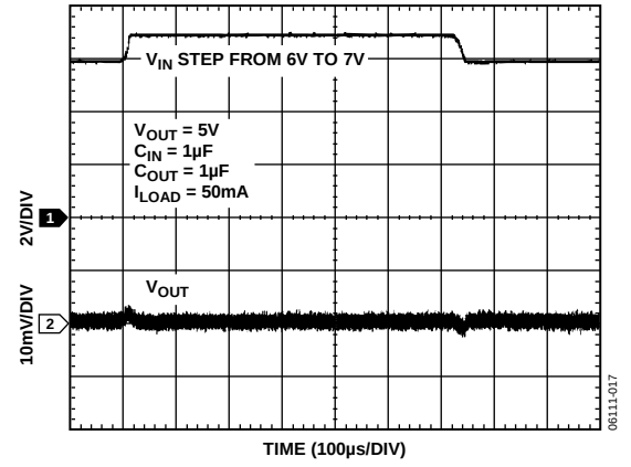
Figure 17. Line Transient Response
