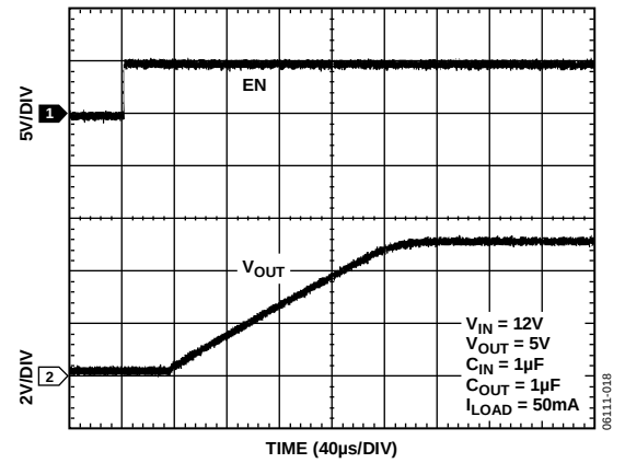
Figure 18. Start-Up Time
