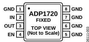
Figure 3. 8-Lead MSOP
