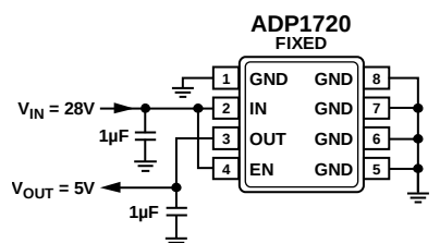
Figure 1. ADP1720 with Fixed Output Voltage, 5.0 V
