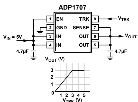
Figure 2. ADP1707 with Output Voltage Tracking
