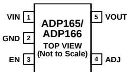
Figure 5. 5-Lead TSOT, Adjustable Output Pin Configuration
