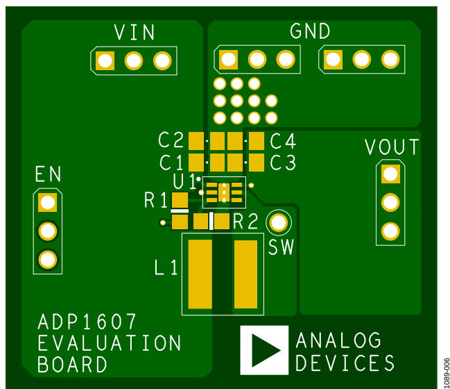
Figure 6. ADP1607 Boost Application Printed Circuit Board (PCB) Top Layer
