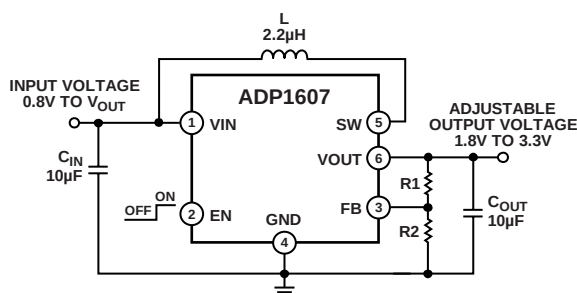
Figure 1. Step-Up Regulator Configuration
