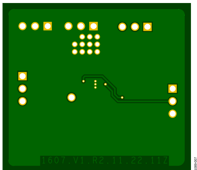
Figure 7. ADP1607 Boost Application PCB Bottom Layer
