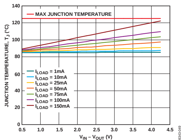
Figure 46. WLCSP, 100 mm² of PCB Copper, Board Temperature = 85°C
