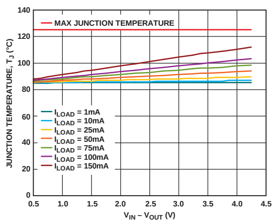
Figure 39. TSOT, 100 mm² of PCB Copper, Board Temperature = 85°C
