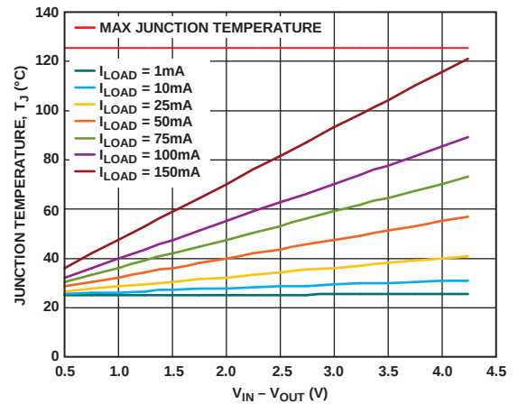
Figure 40. WLCSF, 500 mm² of PCB Copper, T_A = 25^\circ\text{C}
