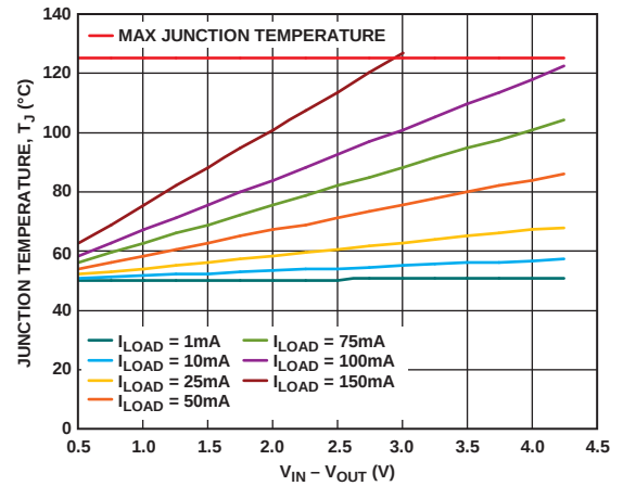
Figure 38. TSOT, 0 mm² of PCB Copper, T_A = 50^\circ\text{C}
