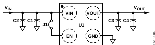
Figure 4. Evaluation Board Schematic, WLCSP
