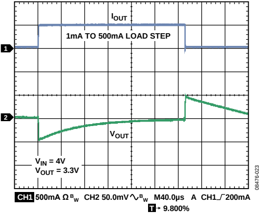
Figure 25. Load Transient Response, C_{OUT} = 4.7 \mu F
