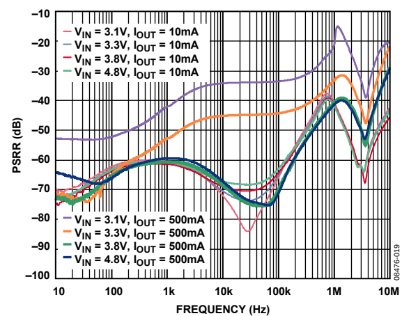
Figure 21. Power Supply Rejection Ratio vs. Headroom Voltage ( V_{IN} - V_{OUT} ), V_{OUT} = 2.8\text{ V}
