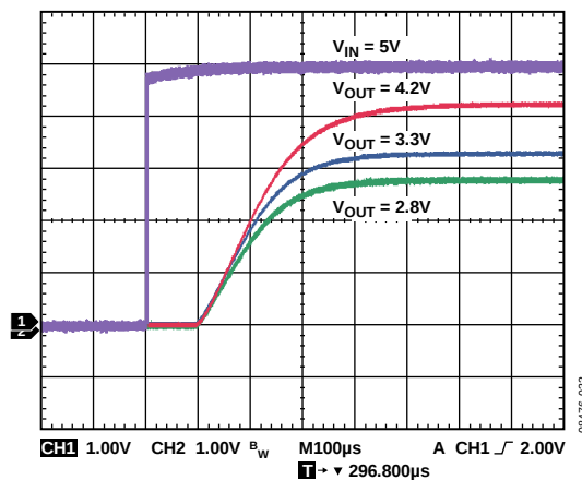
Figure 35. Typical Start-Up Time
