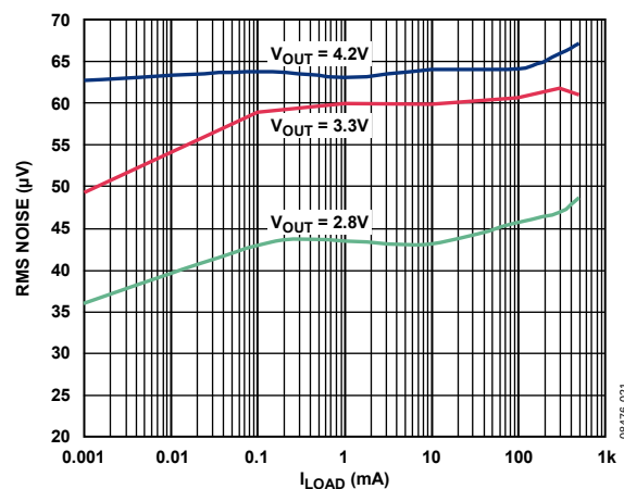
Figure 23. Output Noise vs. Load Current and Output Voltage, V_{IN} = 5\text{ V}
