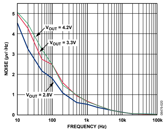
Figure 22. Output Noise Spectrum, V_{IN} = 5\text{ V}
