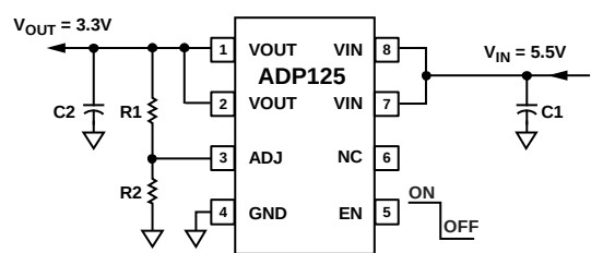
Figure 2. ADP125 with Adjustable Output Voltage
