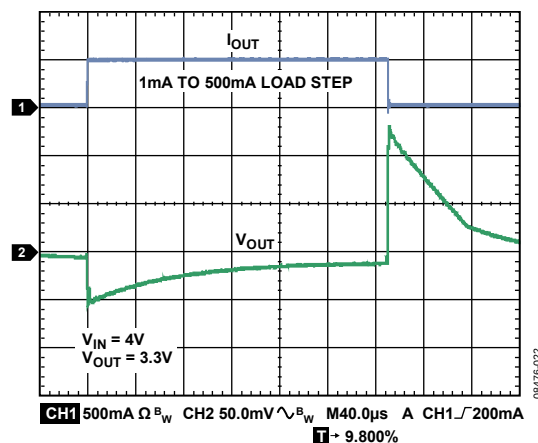
Figure 24. Load Transient Response, C_{OUT} = 1\text{ μF}
