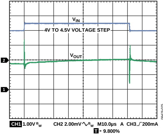
Figure 27. Line Transient Response, Load Current = 500 mA
