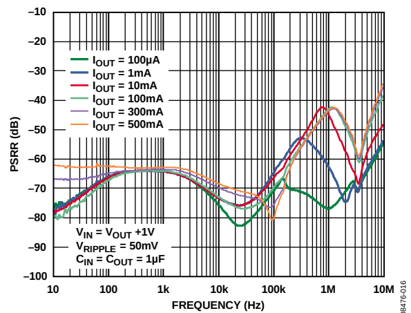
Figure 18. Power Supply Rejection Ratio vs. Frequency, V_{OUT} = 3.3V , V_{IN} = 4.3V
