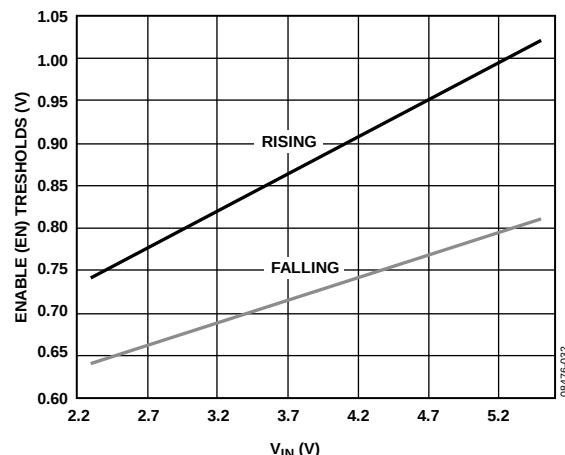
Figure 34. Typical EN Pin Thresholds vs. Input Voltage
