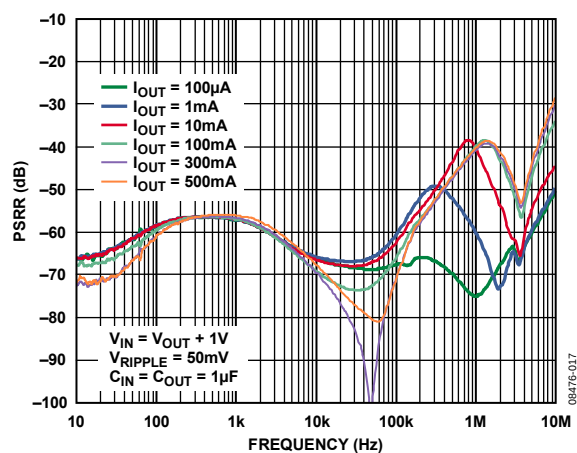
Figure 19. Power Supply Rejection Ratio vs. Frequency, V_{OUT} = 4.2\text{ V} , V_{IN} = 5.2\text{ V}
