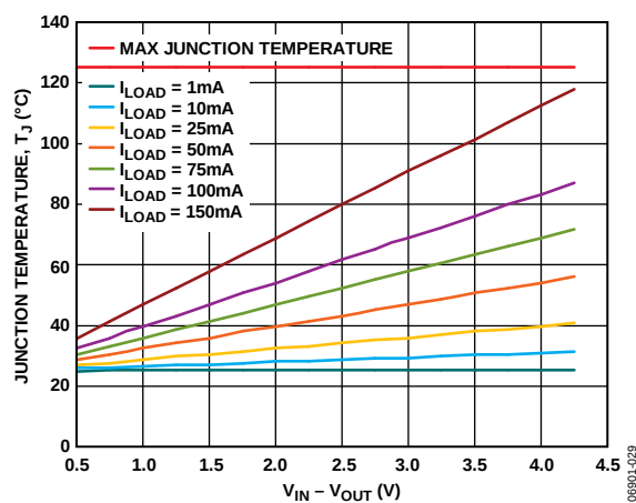
Figure 35. TSOT, 100 mm² of PCB Copper, T_A = 25^\circ\text{C}
