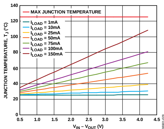
Figure 34. TSOT, 500 mm² of PCB Copper, T_A = 25^\circ\text{C}
