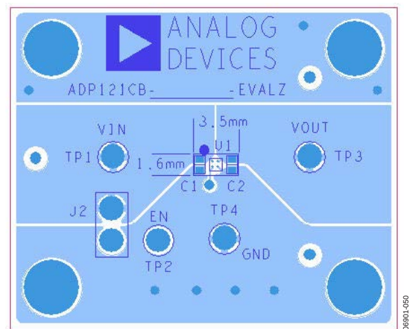
Figure 49. Example of WLCSP PCB Layout—Top Side
