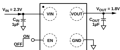
Figure 2. ADP121 WLCSP with Fixed Output Voltage, 1.8 V
