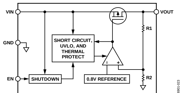
Figure 27. Internal Block Diagram
