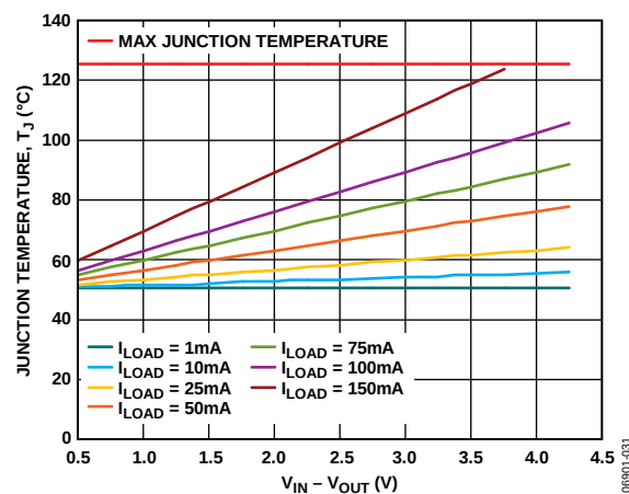
Figure 37. TSOT, 500 mm² of PCB Copper, T_A = 50^\circ\text{C}
