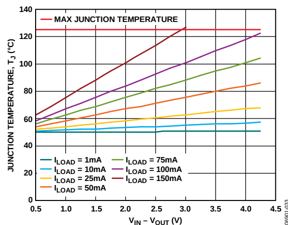
Figure 39. TSOT, 0 mm² of PCB Copper, T_A = 50^\circ\text{C}
