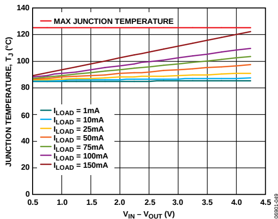
Figure 47. WLCSP, 100 mm² of PCB Copper, Board Temperature = 85°C
