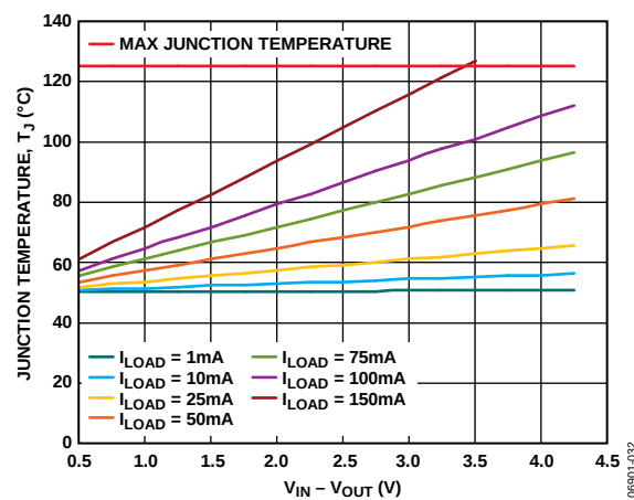
Figure 38. TSOT, 100 mm² of PCB Copper, T_A = 50^\circ\text{C}
