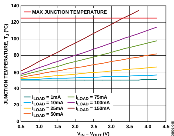
Figure 43. WLCSP, 500 mm² of PCB Copper, T_A = 50^\circ\text{C}
