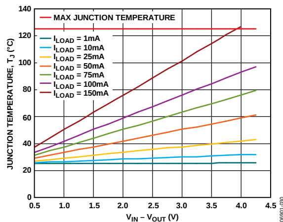
Figure 36. TSOT, 0 mm² of PCB Copper, T_A = 25^\circ\text{C}
