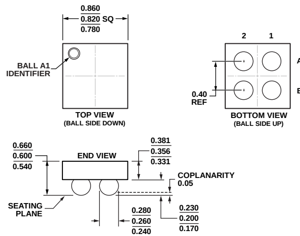
Figure 52. 4-Ball Wafer Level Chip Scale- Package [WLCSP] (CB-4-2)
