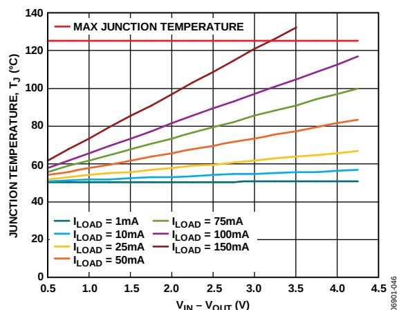
Figure 44. WLCSP, 100 mm² of PCB Copper, T_A = 50^\circ\text{C}
