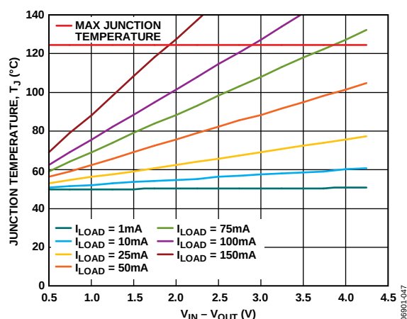
Figure 45. WLCSP, 0 mm² of PCB Copper, T_A = 50^\circ\text{C}
