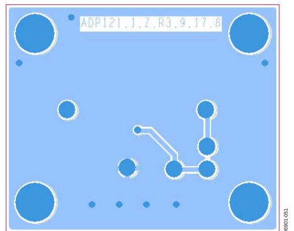
Figure 50. Example of WLCSP PCB Layout—Bottom Side
