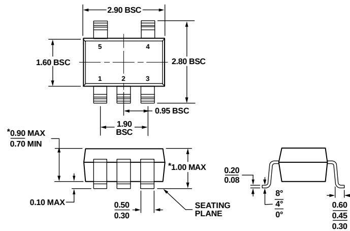
*COMPLIANT TO JEDEC STANDARDS MO-193-AB WITH THE EXCEPTION OF PACKAGE HEIGHT AND THICKNESS. Figure 51. 5-Lead Thin Small Outline Transistor Package [TSOT] (UJ-5)
