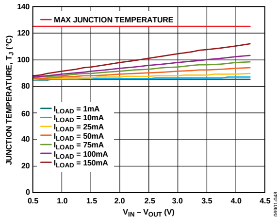
Figure 46. TSOT, 100 mm² of PCB Copper, Board Temperature = 85°C
