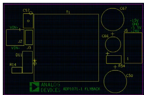
Figure 18. Silkscreen Top
