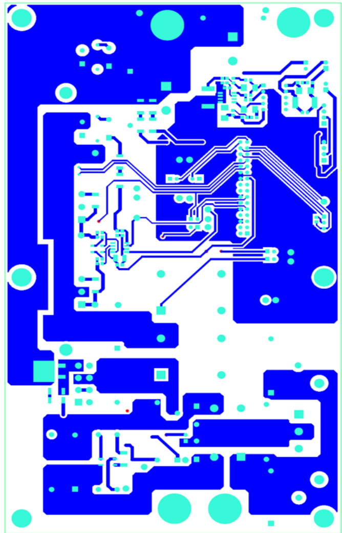
Figure 13 - Layout, Bottom layer
