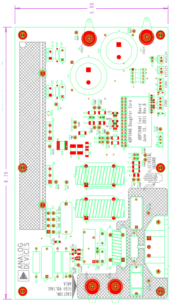
Figure 10 – Layout, Top Silkscreen
