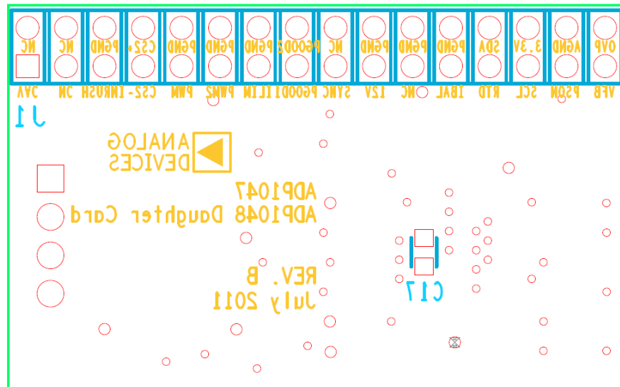
Figure 16 – Bottom Silkscreen
