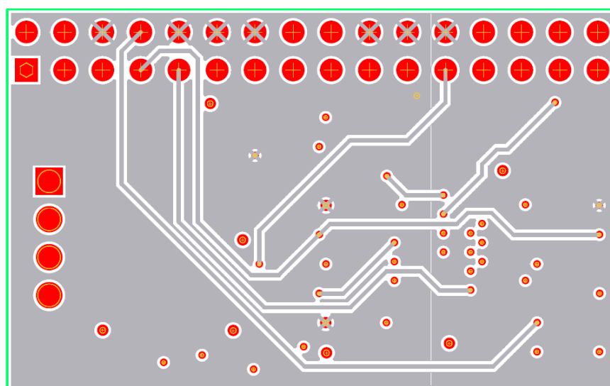
Figure 19 – inner layer2 layout
