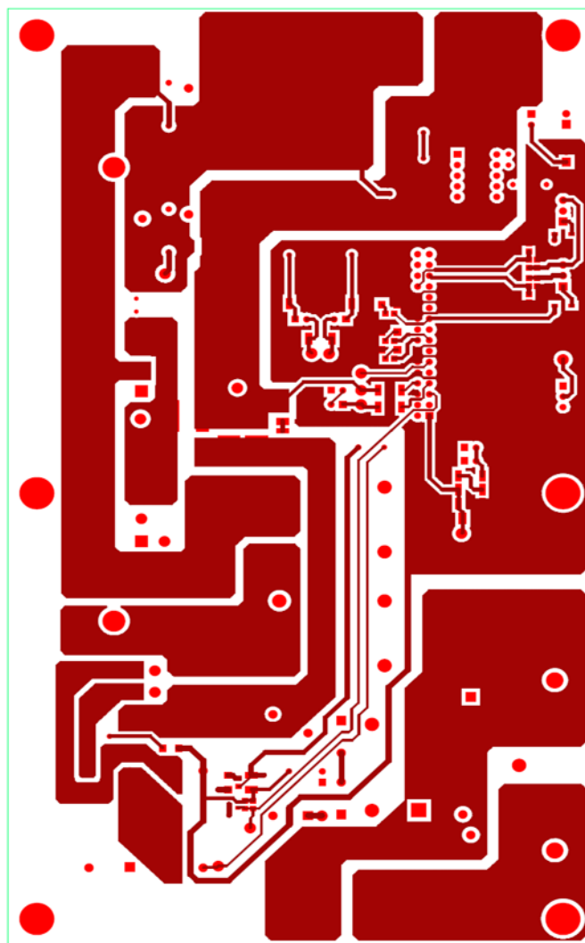
Figure 11 - Layout, Top layer
