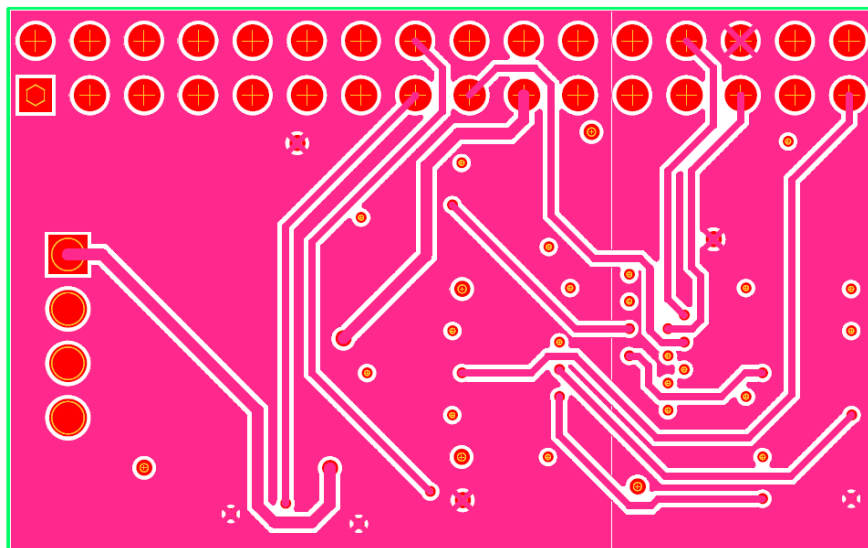
Figure 18 – Inner layer1 layout
