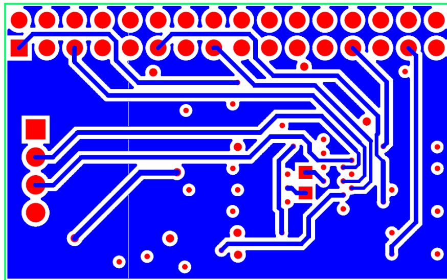
Figure 17 – Bottom layer
