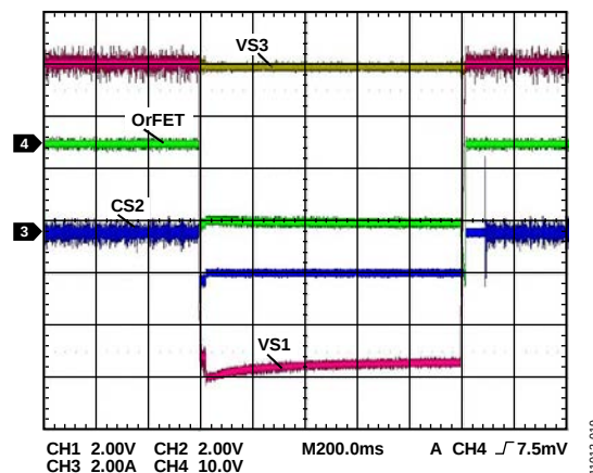
Figure 29. Internal Short Circuit (Yellow Is Bus Voltage; Red Is VS1 Voltage; Green Is OrFET Control Signal; Blue Is Load Current)
