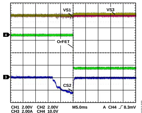
Figure 30. Light Load Mode (Yellow Is Bus Voltage; Red Is VS1 Voltage; Green Is OrFET Control Signal; Blue Is Load Current)
