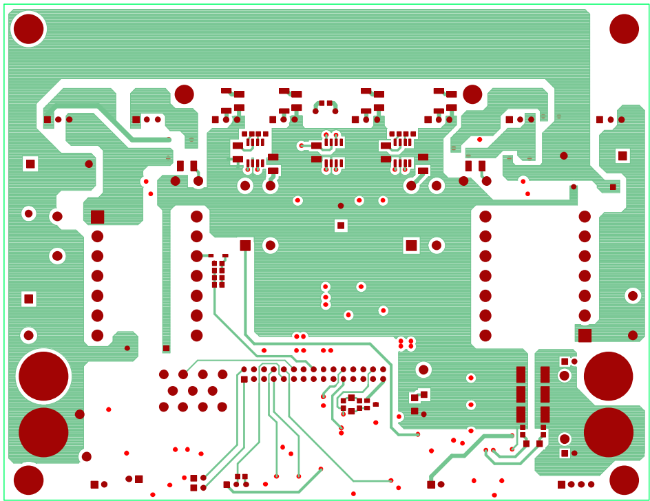
Figure 82. Layout, Bottom Layer, 6.5 in × 5 in
