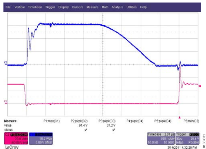
Figure 32. Synchronous Rectifier and Freewheeling MOSFET PIV at 25 A Load, 350 V DC
