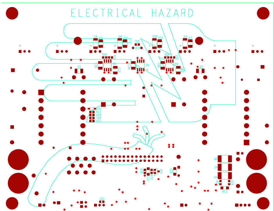
Figure 83. Layout, Bottom Layer Silkscreen, 6.5 in × 5 in
