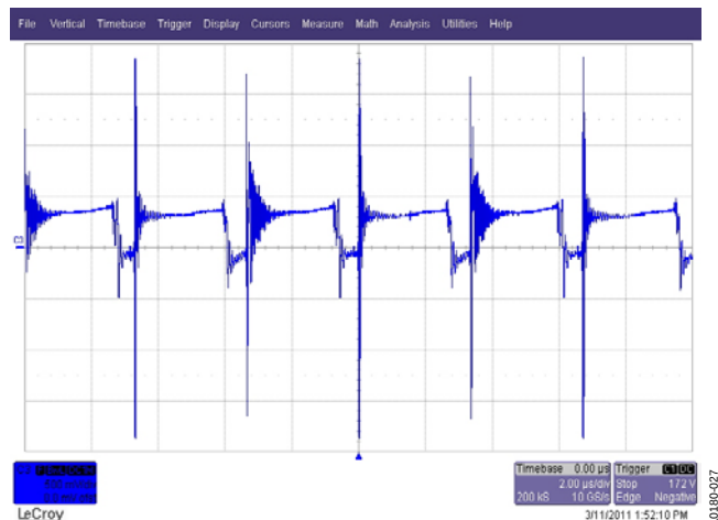
CS1 PIN VOLTAGE AND CURRENT BALANCING OF PHASES
