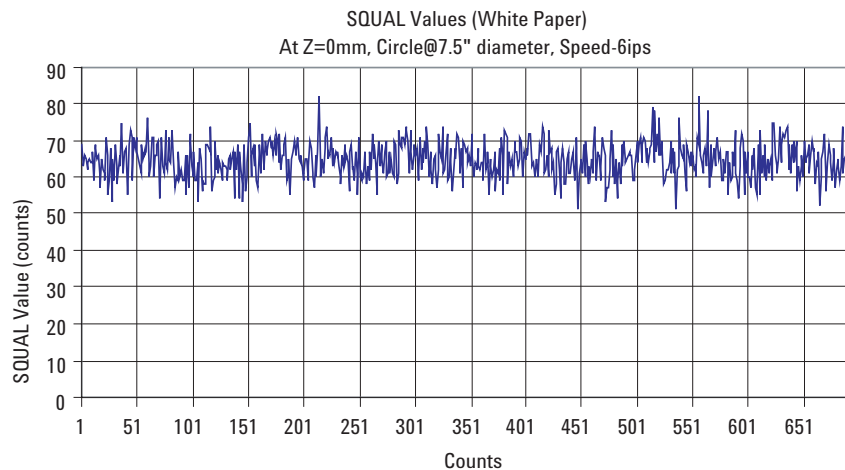
Figure 27. SQUAL Values at 2000dpi (White Paper)
