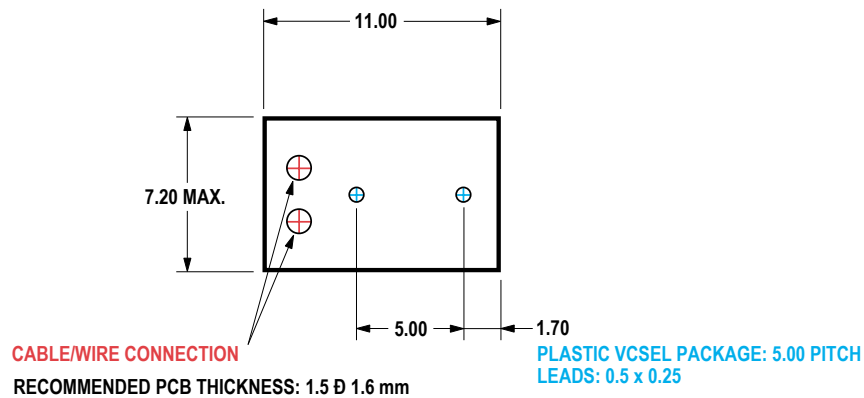
Figure 32. Suggested ADNV-6340 PCB mounting guide.
