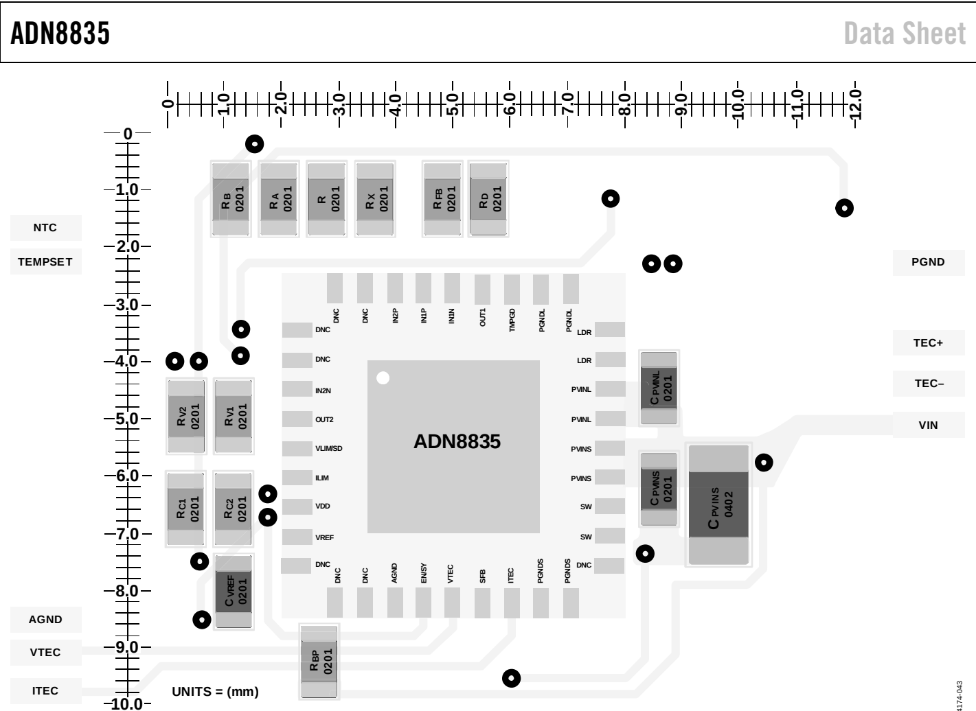
Figure 43. Example PCB Layout Using Two Layers (Bottom Layer Only)
