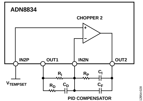
Figure 35. Implementing a PID Compensation Loop
