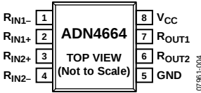
Figure 4. Pin Configuration
