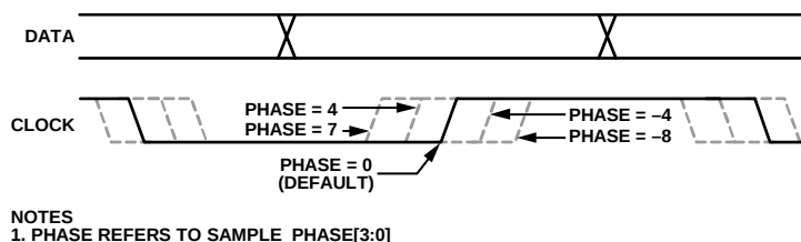
Figure 26. Data vs. Sampling Clock
