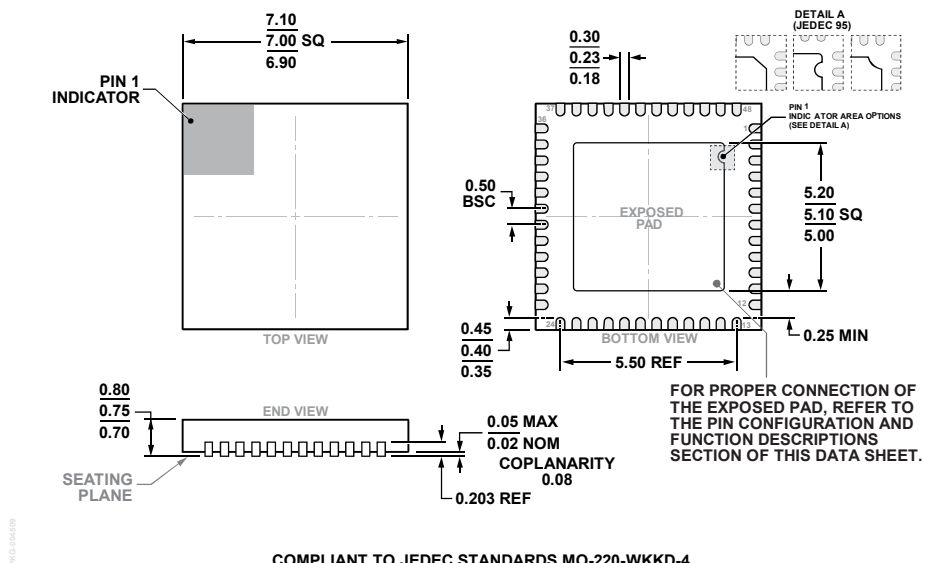
Figure 14. 48-Lead Lead Frame Chip Scale Package [LFCSP] 7 mm × 7 mm Body and 0.75 mm Package Height (CP-48-4)
