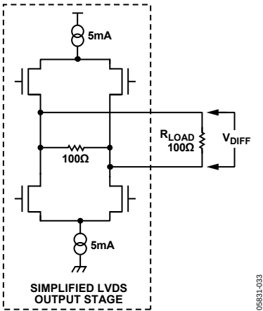
Figure 4. Differential Output Stage
