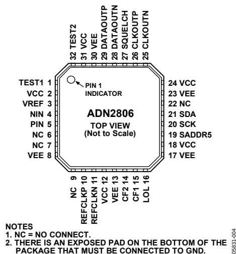
Figure 5. Pin Configuration
