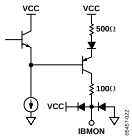
Figure 27. Equivalent Circuit of the IBMON Pin
