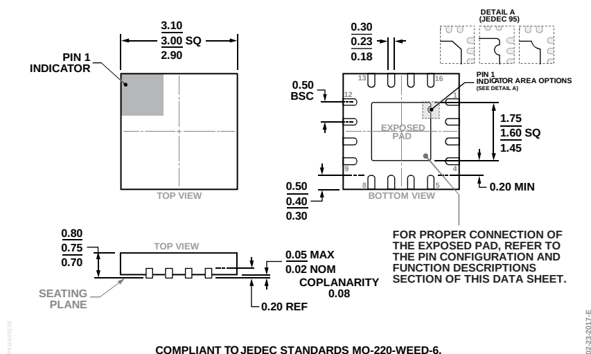
Figure 41. 16-Lead Lead Frame Chip Scale Package [LFCSP] 3 mm x 3 mm Body and 0.75 mm Package Height (CP-16-22) Dimensions shown in millimeters
