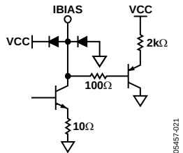
Figure 26. Equivalent Circuit of the IBIAS Pin
