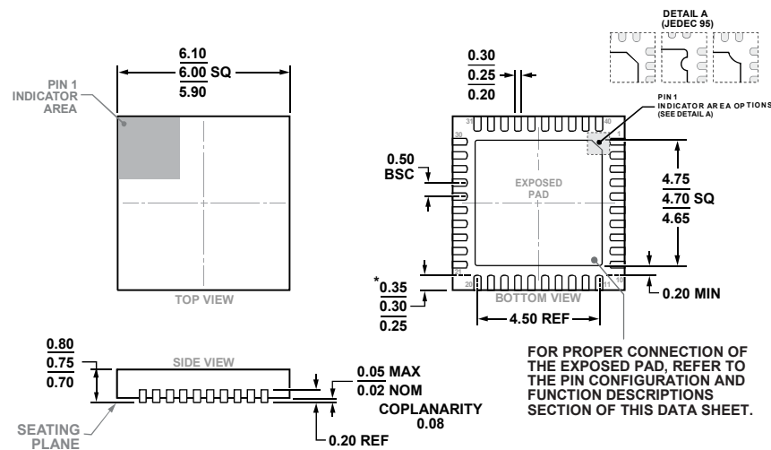
Figure 47. 40-Lead Lead Frame Chip Scale Package [LFCSP] 6 mm × 6 mm Body and 0.75 mm Package Height (CP-40-27)
