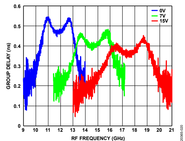
Figure 22. Group Delay vs. RF Frequency at Various VTUNE
