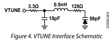
Figure 4. VTUNE Interface Schematic
