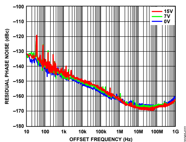
Figure 24. Residual Phase Noise vs. Offset Frequency at Various VTUNE
