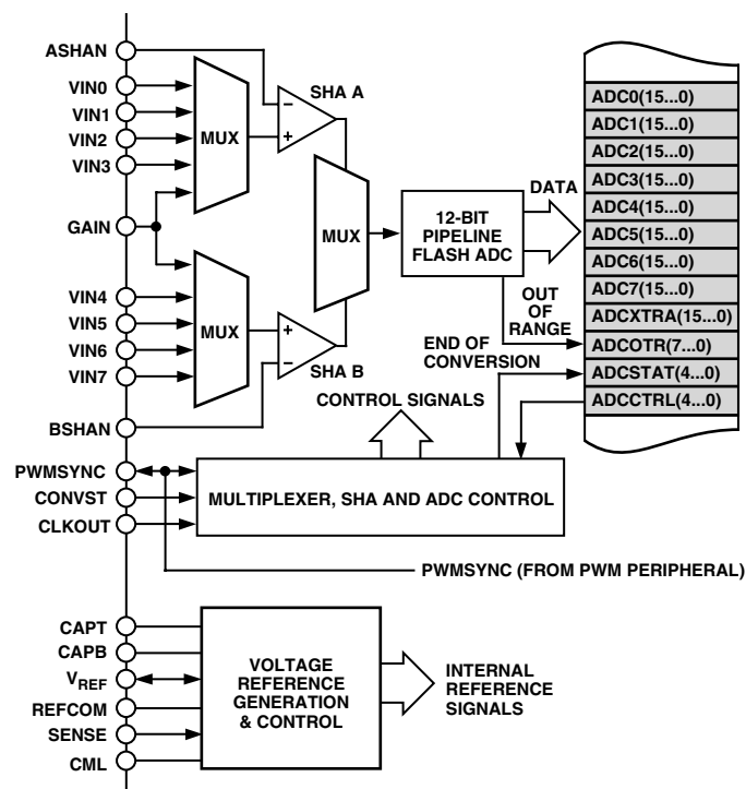
Figure 16. Functional Block Diagram of the ADC System of the ADC401
