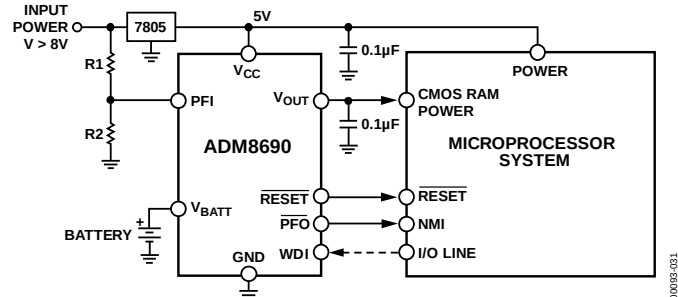
Figure 31. ADM8690 Typical Application, Circuit B
