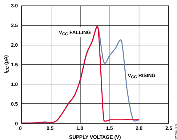
Figure 9. Supply Current ( I_{CC} ) vs. Supply Voltage, V_{CC} < 2\text{V}
