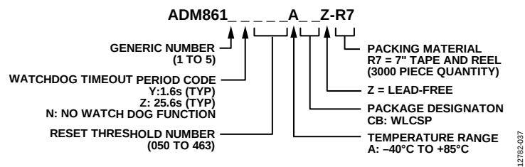
Figure 36. Ordering Code Structure
