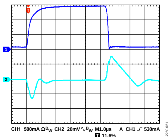
Figure 51. Load Transient Response, I_{LOAD} = 100\text{ mA} to 1.6\text{ A} , Adjustable Version, V_{OUT} = 1.2\text{ V} , V_{IN} = 2.5\text{ V} , CH1 = I_{LOAD} , CH2 = V_{OUT}
