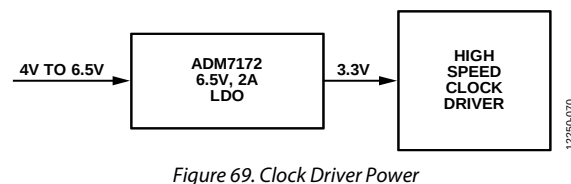
Figure 69. Clock Driver Power
