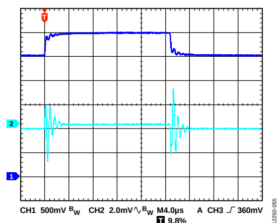
Figure 55. Line Transient Response, 2.5 V to 3 V, I_{LOAD} = 2 A, Adjustable Version, V_{OUT} = 1.2 V, CH1 = V_{IN} , CH2 = V_{OUT}
