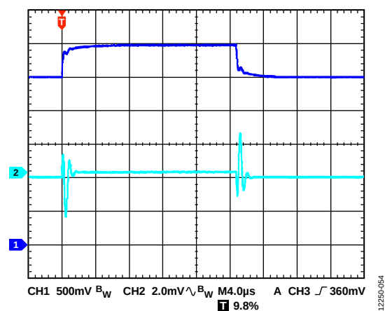
Figure 54. Line Transient Response, 2.5 V to 3 V, I_{LOAD} = 500 mA, Adjustable Version, V_{OUT} = 1.2 V, CH1 = V_{IN} , CH2 = V_{OUT}
