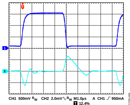
Figure 58. Output Transient Response, V_{\text{OUT}} = 5\text{ V} , C_{\text{OUT}} = 4.7\text{ }\mu\text{F}
