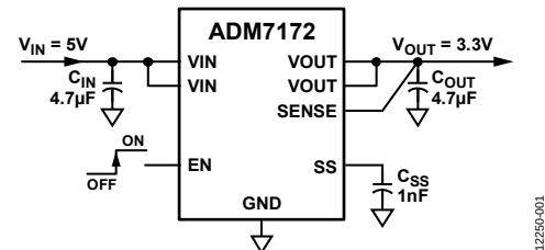
Figure 1. ADM7172 with Fixed Output Voltage, 3.3 V
