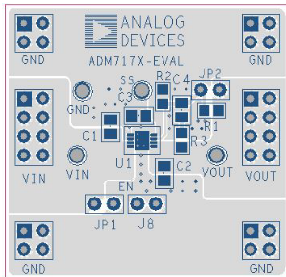
Figure 71. Example LFCSP PCB Layout
