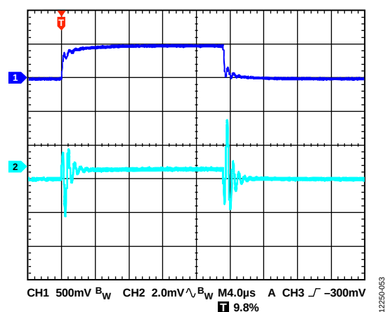
Figure 53. Line Transient Response, 6 V to 6.5 V, I_{LOAD} = 2 A, V_{OUT} = 5 V, CH1 = V_{IN} , CH2 = V_{OUT}
