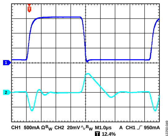
Figure 49. Load Transient Response, I_{LOAD} = 100\text{ mA} to 1.6\text{ A} , V_{OUT} = 5\text{ V} , V_{IN} = 5.5\text{ V} , CH1 = I_{LOAD} , CH2 = V_{OUT}
