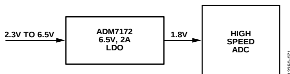
Figure 70. High Speed ADC Power
