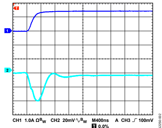
Figure 2. Transient Response (Trace 2), 1 mA to 1.5 A Load Step in 400 ns (Trace 1)
