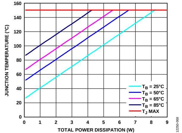
Figure 67. LFCSP Power Dissipation for Various Board Temperatures
