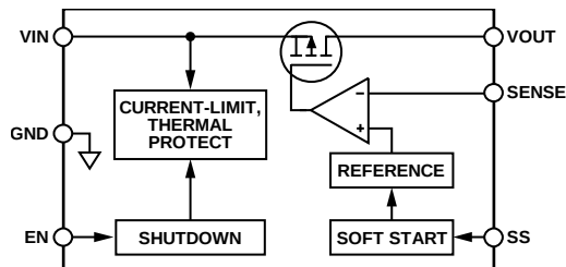
Figure 54. Internal Block Diagram
