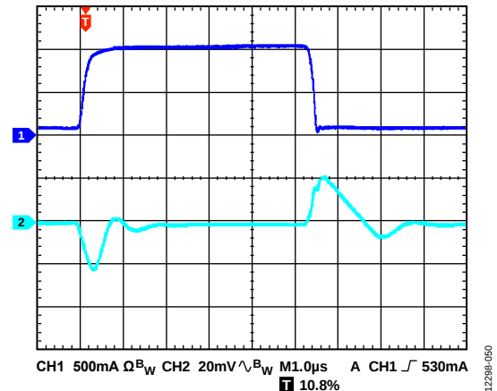
Figure 50. Load Transient Response, I_{LOAD} = 10mA to 1 A, Adjustable Version, V_{OUT} = 1.2V , V_{IN} = 2.5V , CH1 = I_{LOAD} , CH2 = V_{OUT}
