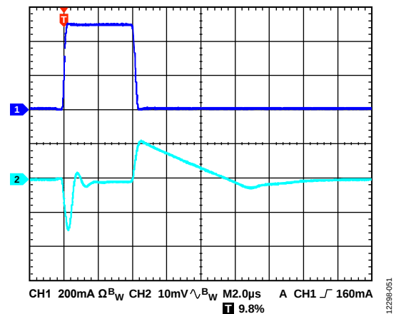
Figure 51. Load Transient Response, I_{LOAD} = 10mA to 500 mA, Adjustable Version, V_{OUT} = 1.2V , V_{IN} = 2.5V , CH1 = I_{LOAD} , CH2 = V_{OUT}
