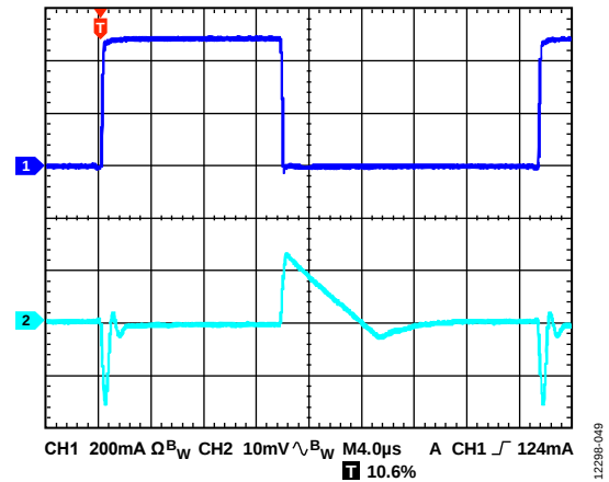
Figure 49. Load Transient Response, I_{LOAD} = 10mA to 500 mA, V_{OUT} = 5V , V_{IN} = 5.5V , CH1 = I_{LOAD} , CH2 = V_{OUT}
