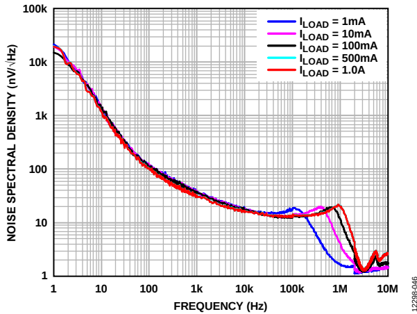
Figure 46. Output Noise Spectral Density, V_{OUT} = 5V
