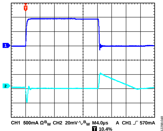
Figure 48. Load Transient Response, I_{LOAD} = 10mA to 1 A, V_{OUT} = 5V , V_{IN} = 5.5V , CH1 = I_{LOAD} , CH2 = V_{OUT}
