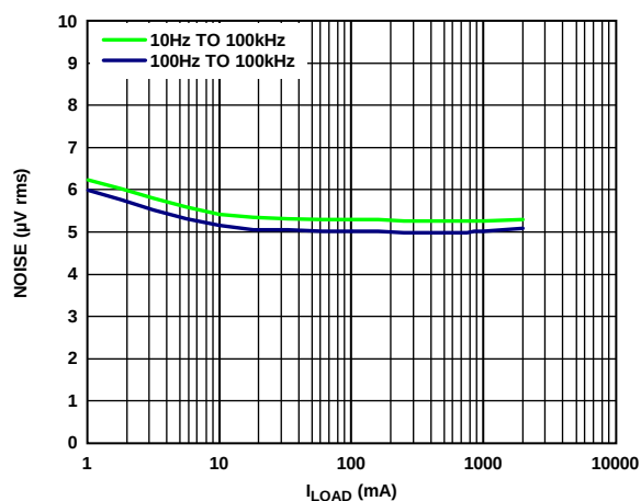
Figure 42. RMS Output Noise vs. Load Current ( I_{LOAD} ), V_{OUT} = 5\text{ V}
