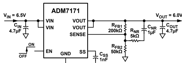
Figure 62. Noise Reduction Modification
