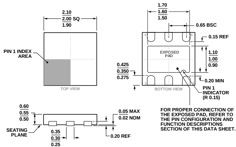
Figure 62. 6-Lead Lead Frame Chip Scale Package [LFCSP_UD] 2.00 mm x 2.00 mm Body, Ultra Thin, Dual Lead (CP-6-3)
