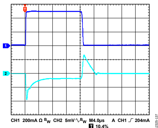
Figure 37. Load Transient Response, I_{LOAD} = 10 mA to 510 mA, V_{OUT} = 1.8 V, V_{IN} = 2.3 V, CH1 = I_{OUT} , CH2 = V_{OUT}
