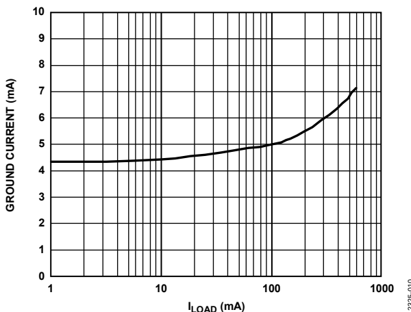
Figure 10. Ground Current vs. Load Current ( I_{LOAD} ), V_{OUT} = 3.3\text{ V}
