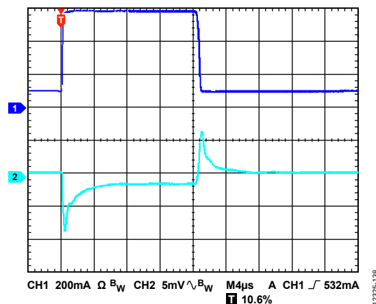
Figure 38. Load Transient Response, I_{LOAD} = 100 mA to 600 mA, V_{OUT} = 1.8 V, V_{IN} = 2.3 V, CH1 = I_{OUT} , CH2 = V_{OUT}
