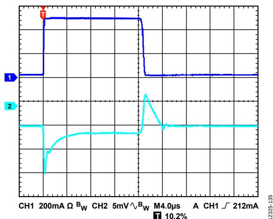
Figure 35. Load Transient Response, I_{LOAD} = 10 mA to 510 mA, V_{OUT} = 3.3 V, V_{IN} = 3.8 V, CH1 = I_{OUT} , CH2 = V_{OUT}
