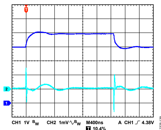
Figure 39. Line Transient Response, 1 V Input Step, I_{LOAD} = 600 mA, V_{OUT} = 3.3 V, V_{IN} = 3.9 V, CH1 = V_{IN} , CH2 = V_{OUT}
