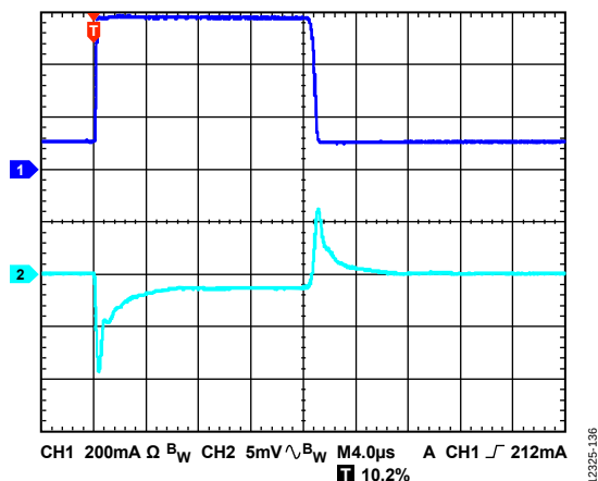
Figure 36. Load Transient Response, I_{LOAD} = 100 mA to 600 mA, V_{OUT} = 3.3 V, V_{IN} = 3.8 V, CH1 = I_{OUT} , CH2 = V_{OUT}
