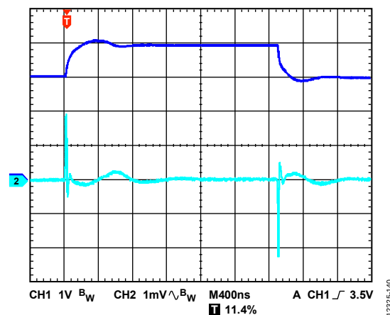
Figure 40. Line Transient Response, 1 V Input Step, I_{LOAD} = 600 mA, V_{OUT} = 1.8 V, V_{IN} = 2.4 V, CH1 = V_{IN} , CH2 = V_{OUT}
